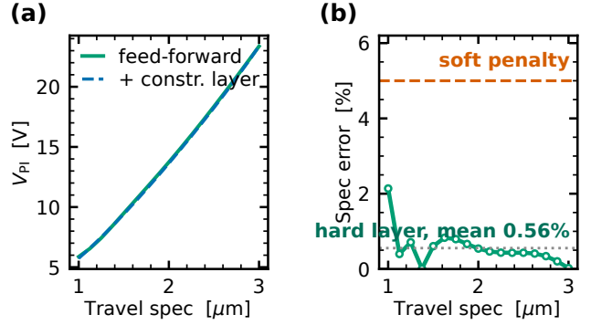
Fig. 5. Specification sweep over the full 1–3 \mu\text{m} range. The differentiable enforcement layer holds specification error at 0.56% mean / 2.14% worst case, against \sim 5\% for a soft penalty.
