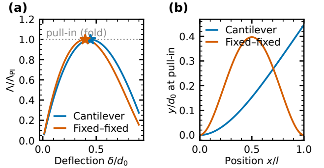
Fig. 1. The fold. Under displacement control the branch is smooth and single-valued through pull-in, where the Jacobian is singular; the deflection shape at the fold is the null vector of (2).
