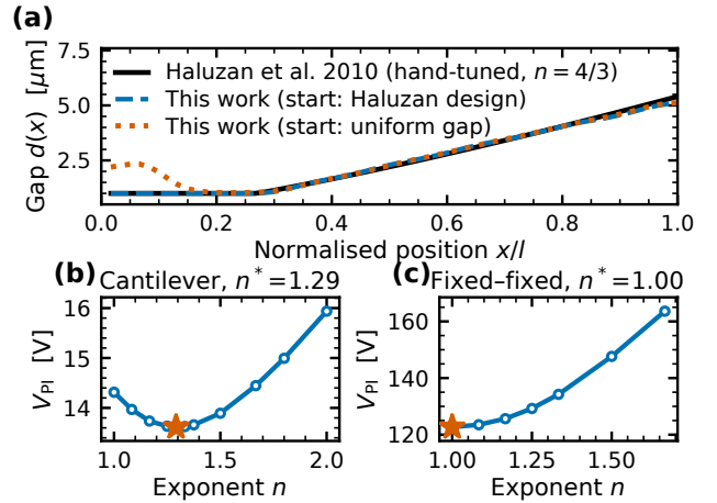
Fig. 4. (a) Free-form profile rediscovered from a uniform-gap start. (b),(c) The optimal exponent reverses between boundary conditions.
