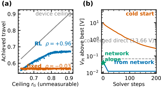
Fig. 6. (a) Achieved travel tracks each device's own hidden ceiling where a fixed gain cannot. (b) Warm-starting from the amortized network.
