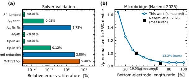
Fig. 3. Error across all validation sources, and the 2025 measured microbridge [5] against our prediction.
