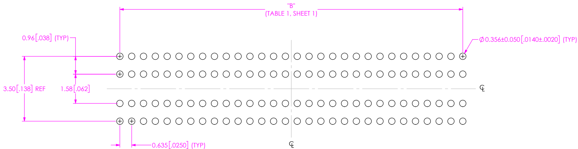
FIG 4 ADM6-30-XX.X-XXX-4-2-A STENCIL SHOWN (TERMINATION STYLE FOR EXISTING CUSTOMERS ONLY)
