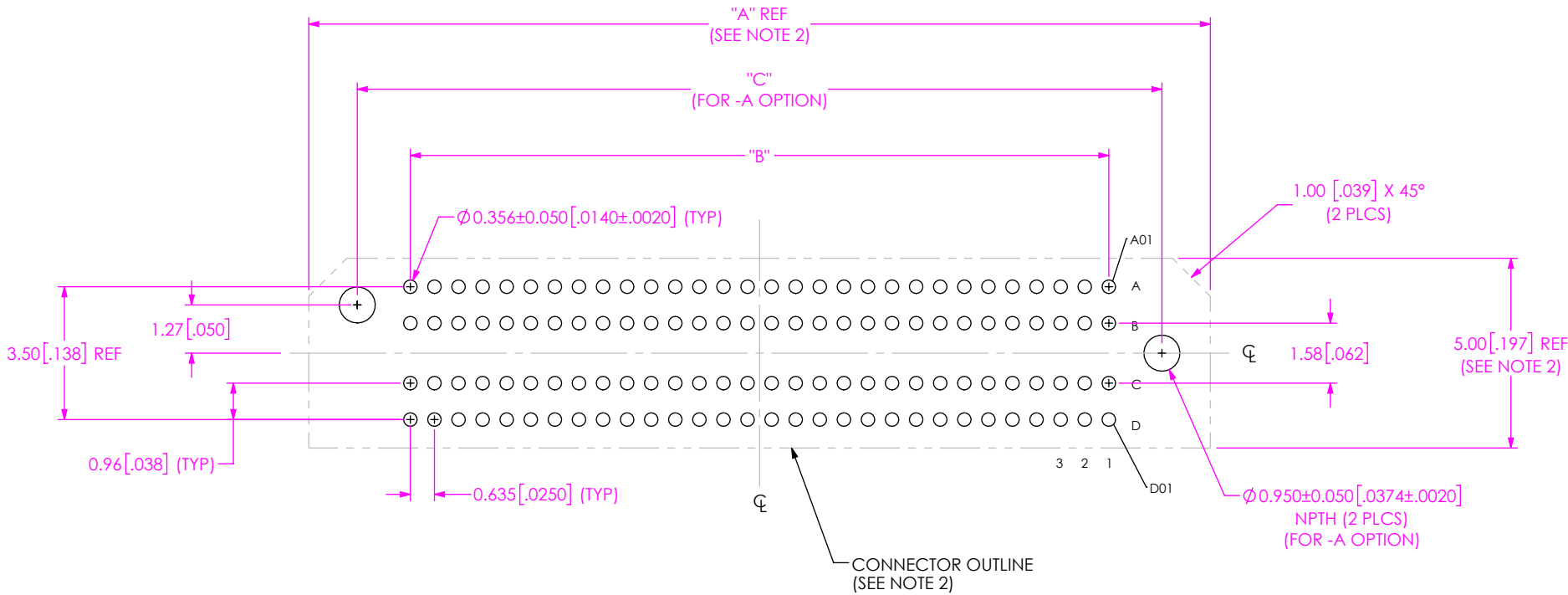
FIG 1 ADM6-30-XX.X-XXX-4-0-A FOOTPRINT SHOWN
