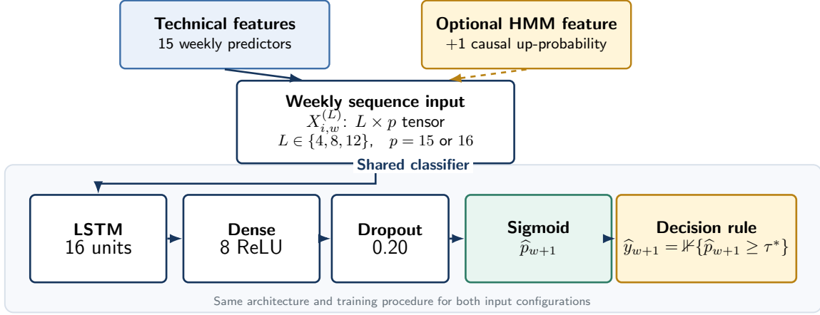
Figure 11: Architecture of the controlled weekly LSTM classifier. The technical-only model receives 15 weekly technical predictors, while the HMM-informed model adds one causal HMM-derived up-probability. Both configurations use the same 16-unit LSTM, eight-unit ReLU dense layer, dropout of 0.20, sigmoid output, and validation-selected classification rule.
