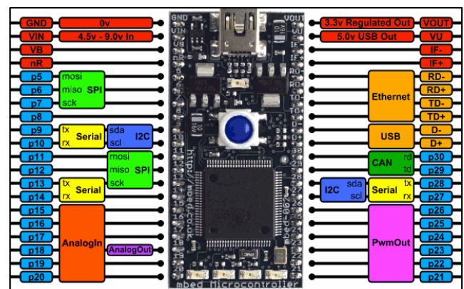
Figure 1: mbed NXP LPC 1768 pinout
