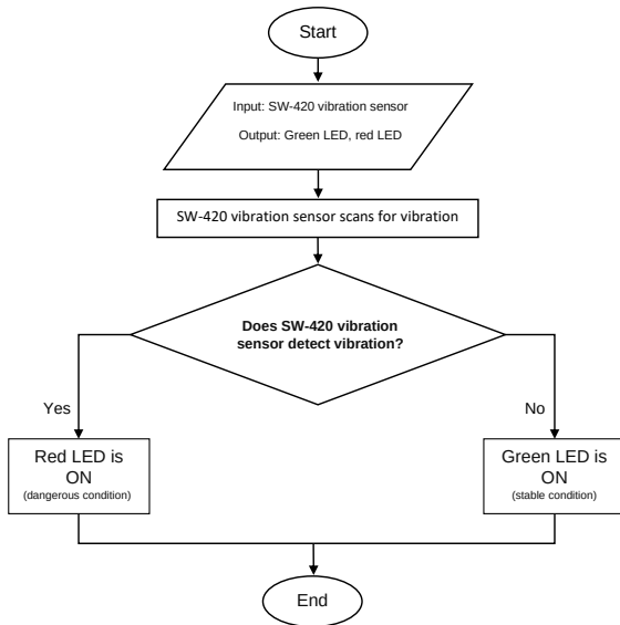
Figure 6: Flowchart of the Landslide Detection System
