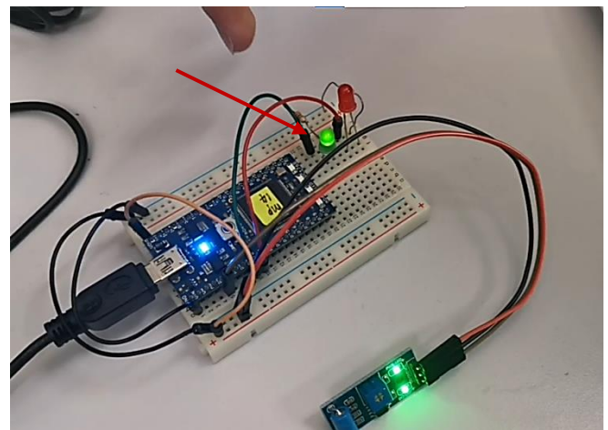
Figure 7: When there is no vibration or shake is detected, the Green LED is ON and Red LED is at OFF state
