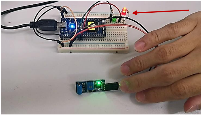
Figure 8: When there is no vibration or shake is detected, the Red LED is ON and Green LED is at OFF state
