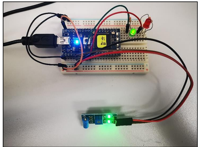
Figure 5: Hardware Construction of the Landslide Detection System
