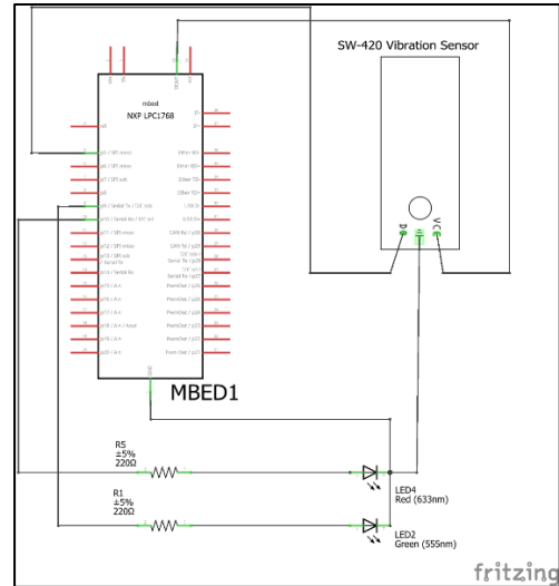
Figure 4: Schematic Circuit designed in Fritzing
