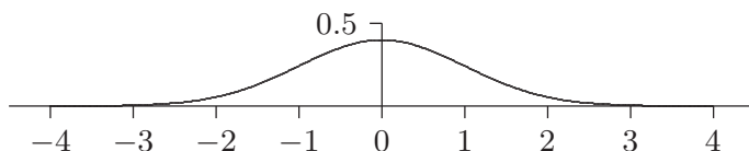
Figure 9.17 The bell curve.
