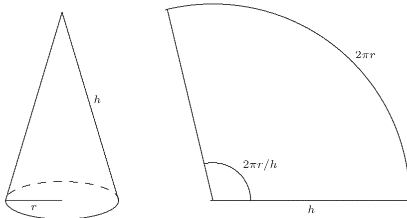
Figure 9.22 The area of a cone.
