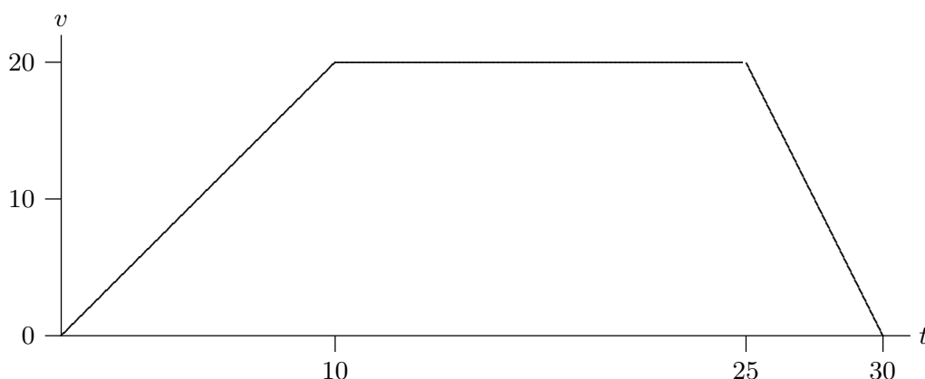
Figure 1.7 A velocity function.
