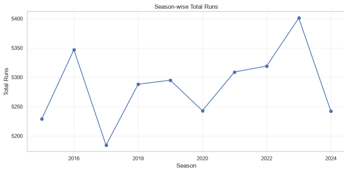
Figure 8. Season-wise Total Runs
