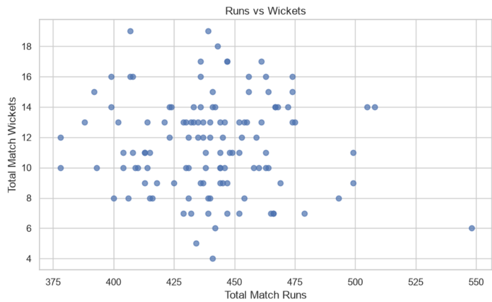
Figure 13. Runs vs Wickets
