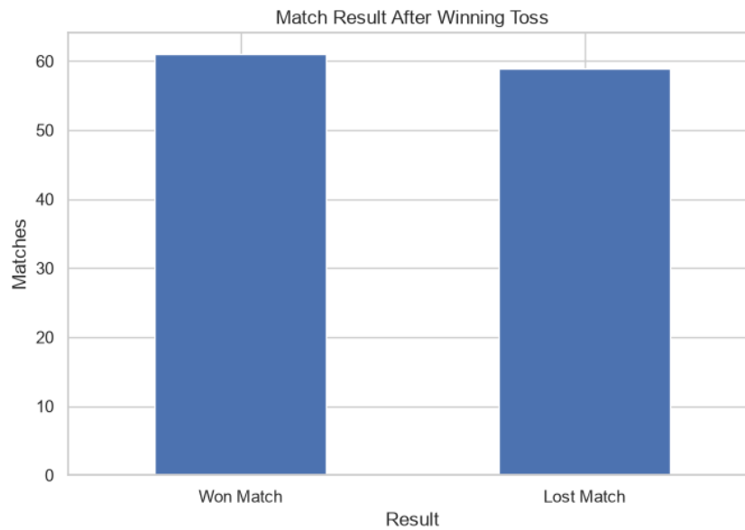
Figure 7. Match Result After Winning Toss
