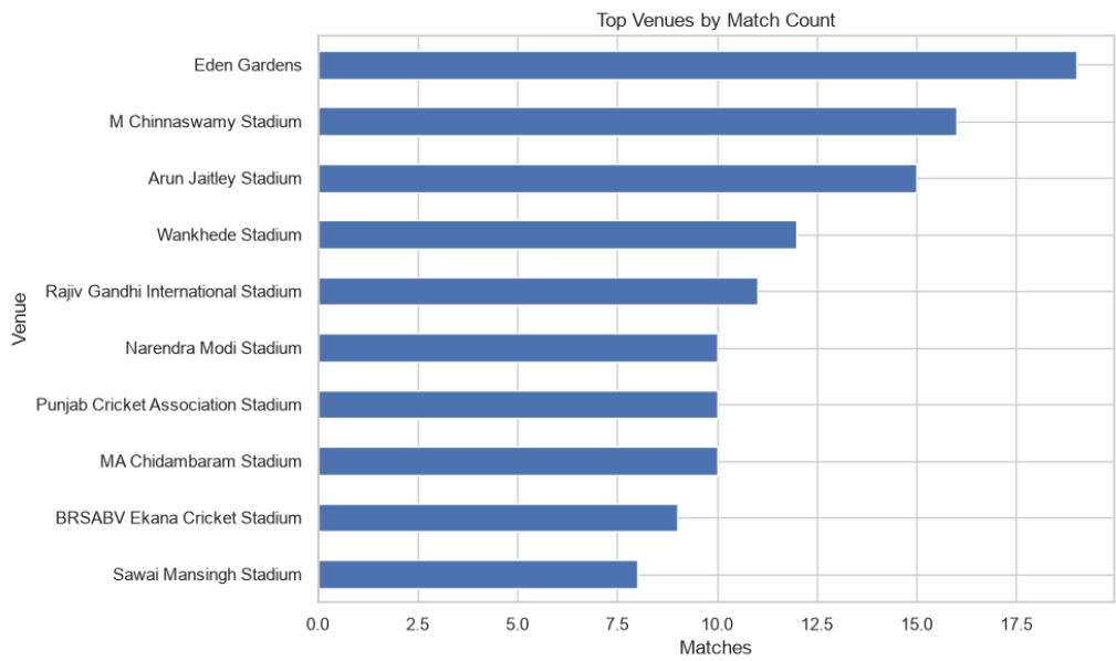
Figure 12. Top Venues by Match Count
