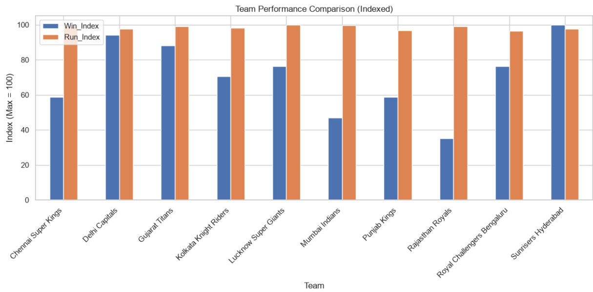
Figure 11. Team Performance Comparison (Indexed)
