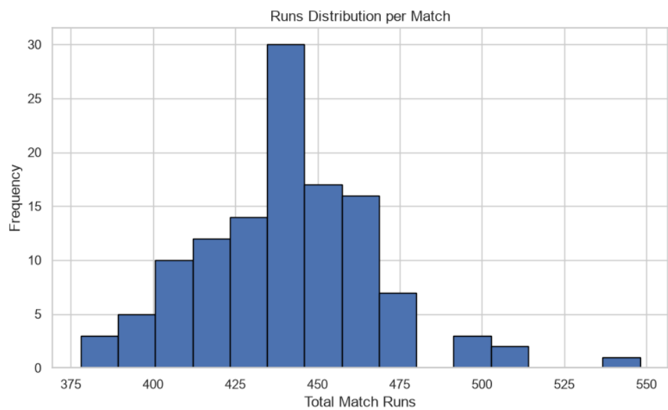
Figure 10. Runs Distribution per Match
