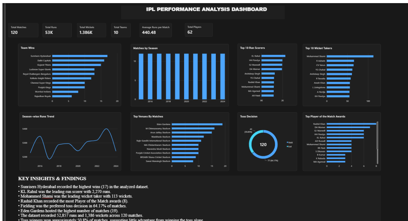
Figure 15. Final IPL Performance Analysis Dashboard
