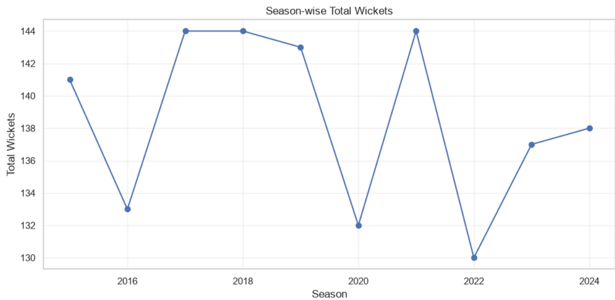
Figure 9. Season-wise Total Wickets
