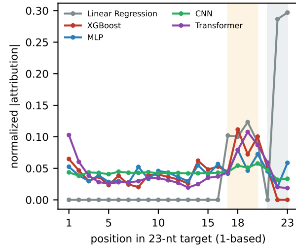
A Cross-model position profile
