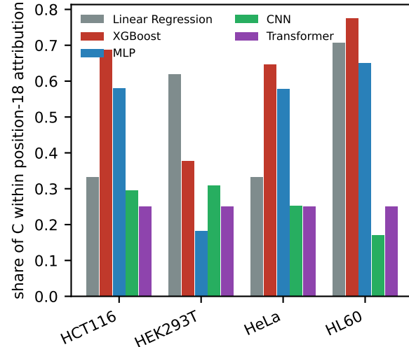
D Model attribution of 18C
