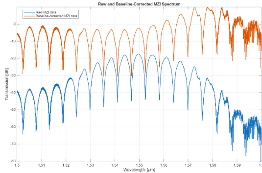
Fig. 10. Baseline corrected experimental data(orange) for MZI with path difference \Delta L = 100\mu\text{m}
