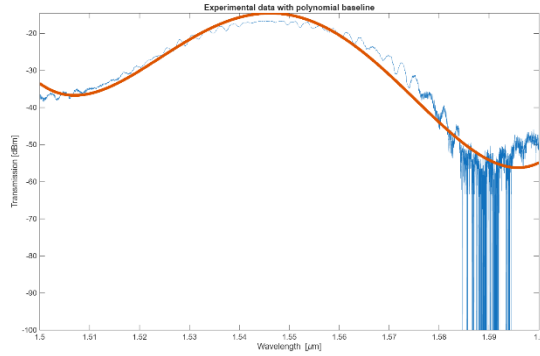
Fig. 9. Fitted 4 th order polynomial for baseline correction
