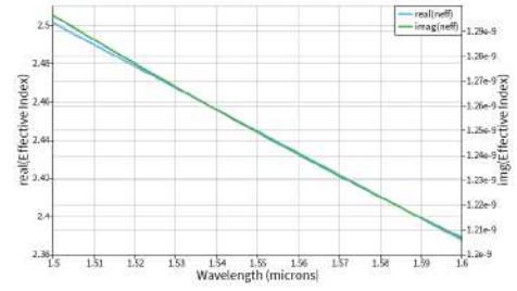
(a) Effective index n_{eff} of quasi-TE mode.
