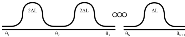
Fig. 2. General structure of optical lattice filter
