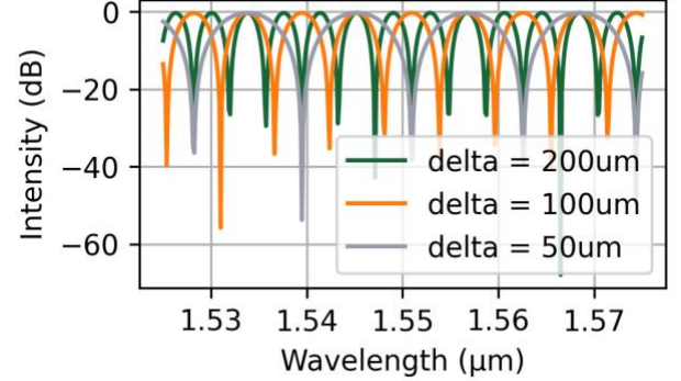
Fig. 7. Transfer function of MZIs
