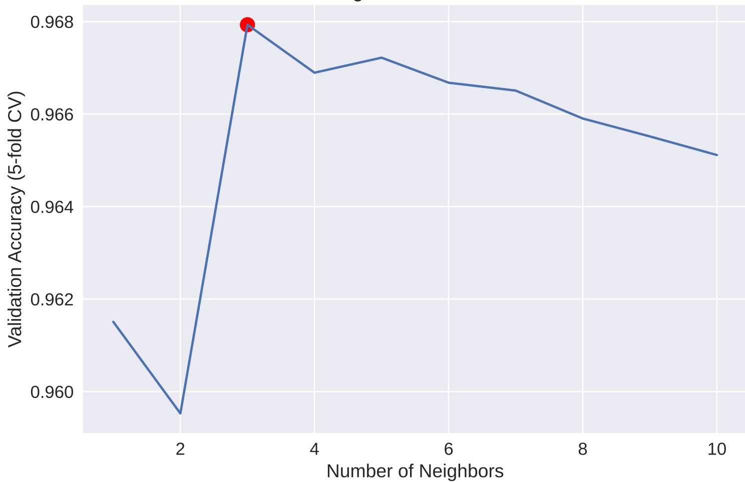
Best Number of Neighbors for KNN - Cross Validation
