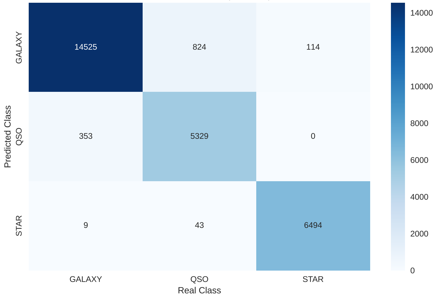
QDA Confusion Matrix (Absolute)
