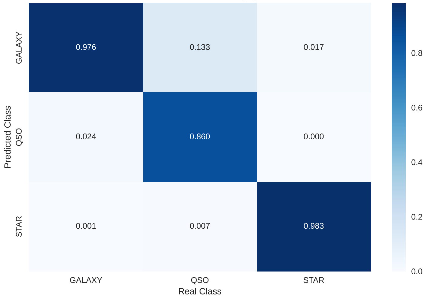
QDA Confusion Matrix (%)
