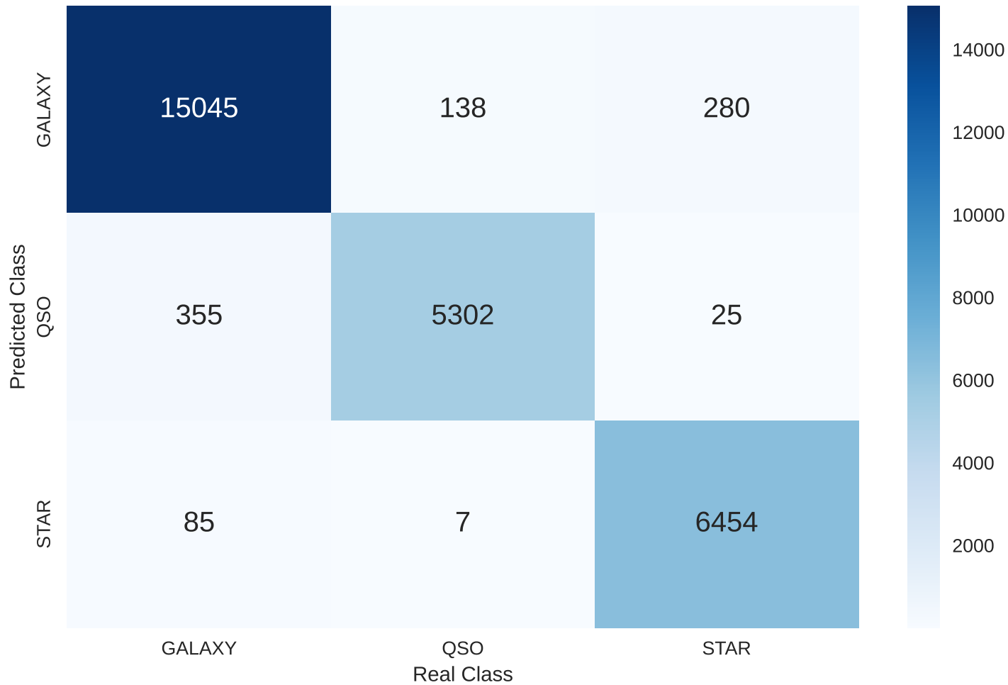
KNN Confusion Matrix (Absolute)
