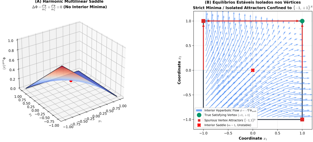
Figure 2: Source figure illustrating harmonic saddle geometry and confinement of isolated stable projected equilibria to Boolean vertices.
