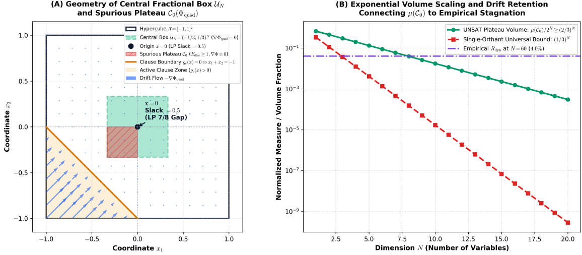
Figure 1: Source figure from the audited CLG-R manuscript illustrating the central fractional box and its exponential-volume scaling. The theorem used in this paper is the deterministic inclusion \mathcal{U}_N \subseteq \mathcal{Z} .
