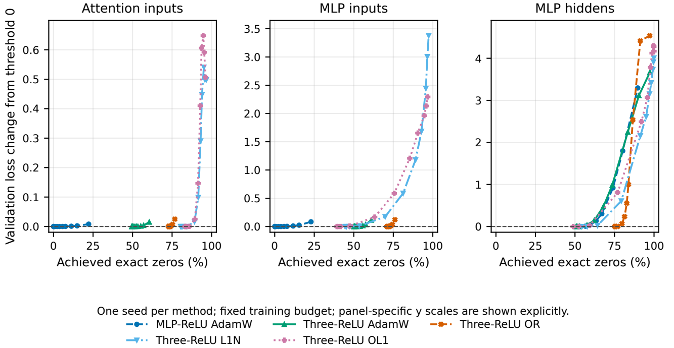
Figure 9: Site-specific clipping frontiers. Validation-loss change is measured from each checkpoint’s own threshold-zero loss, separating clipping fragility from training quality. The panels show that equal near-zero mass does not imply equal removable computation across attention input, MLP input, and MLP hidden.
