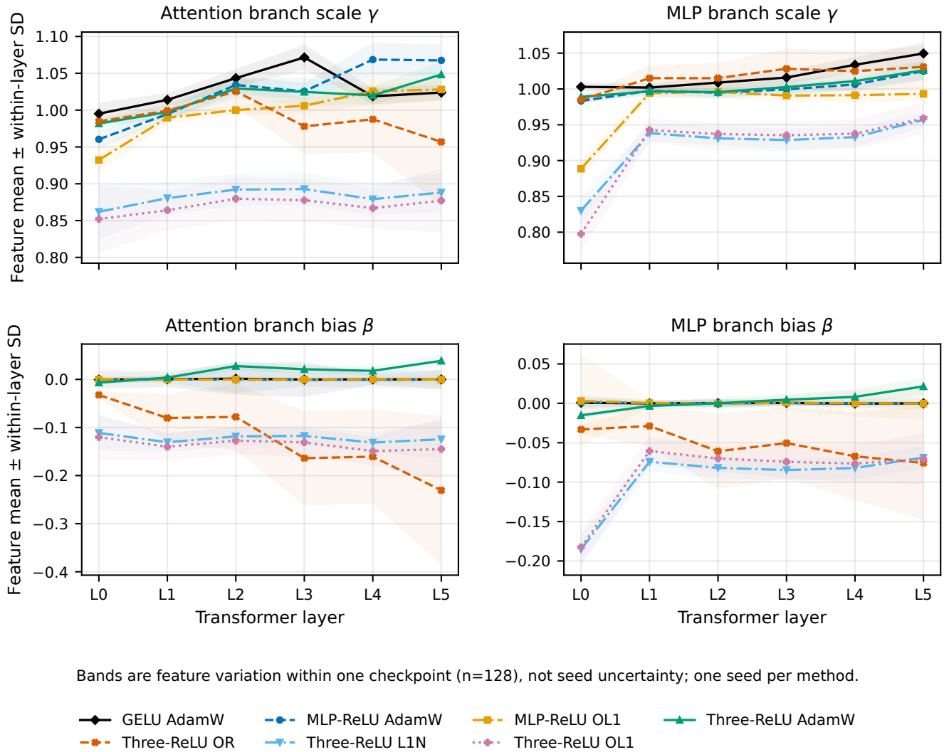
Figure 8: Attention-branch and MLP-branch LayerNorm affine parameters, separated from downstream matrix weights. Negative bias shifts more normalized coordinates below the ReLU threshold; scale changes alter the width of the surviving distribution. Values are associations at the final checkpoint, not a causal decomposition.
