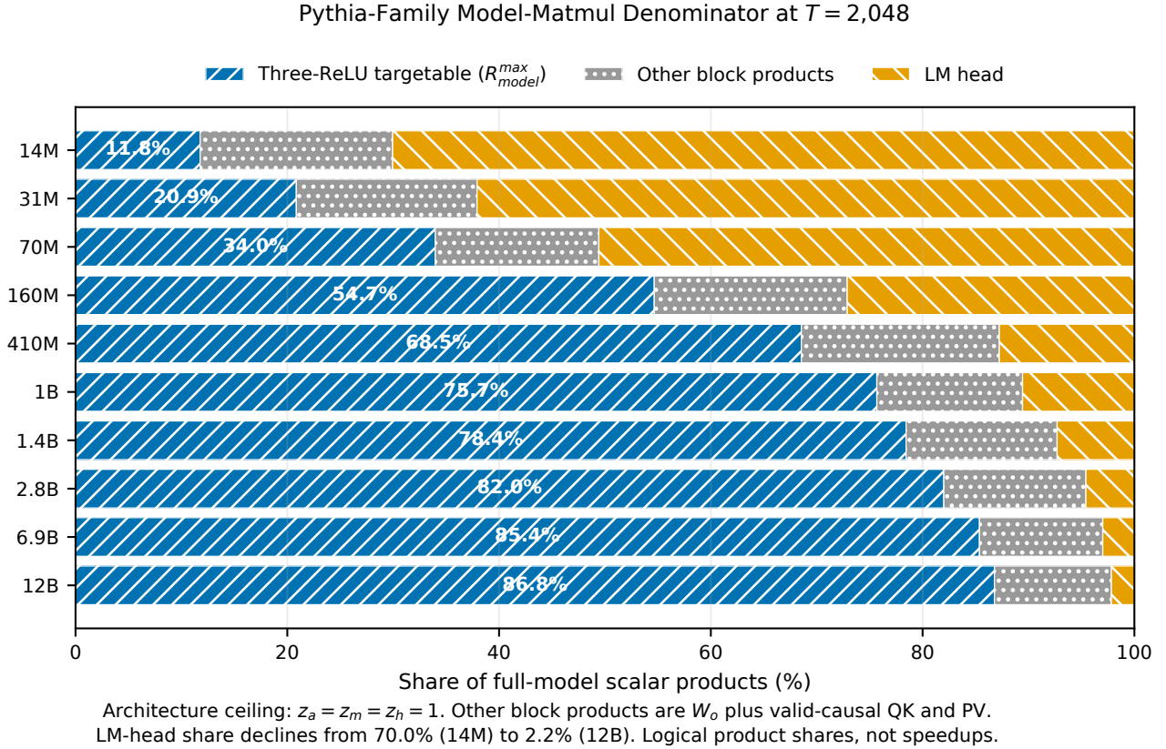
Figure 2: Pythia-family decomposition of the full-model scalar-product denominator at T = 2048 . Blue is the maximum Three-ReLU-targetable share R_{\text{model}}^{\max} ; gray is the untargeted W_o plus valid-causal QK and PV work; orange is the LM head. Every bar assumes z_a = z_m = z_h = 1 , so these are architecture ceilings rather than observed sparsity or speedups.
