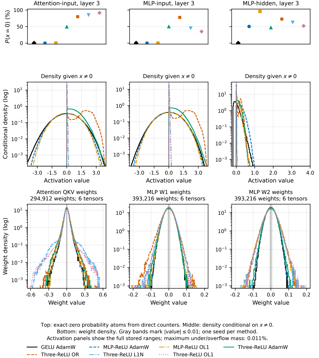
Figure 7: Activation and immediately downstream weight densities for the control ladder, using shared method colors. Pairing each activation with the matrix that consumes it distinguishes hard gates, small-positive reservoirs, and weight adaptation. Exact-zero point masses are reported separately from direct counters rather than inferred from continuous density estimates.
