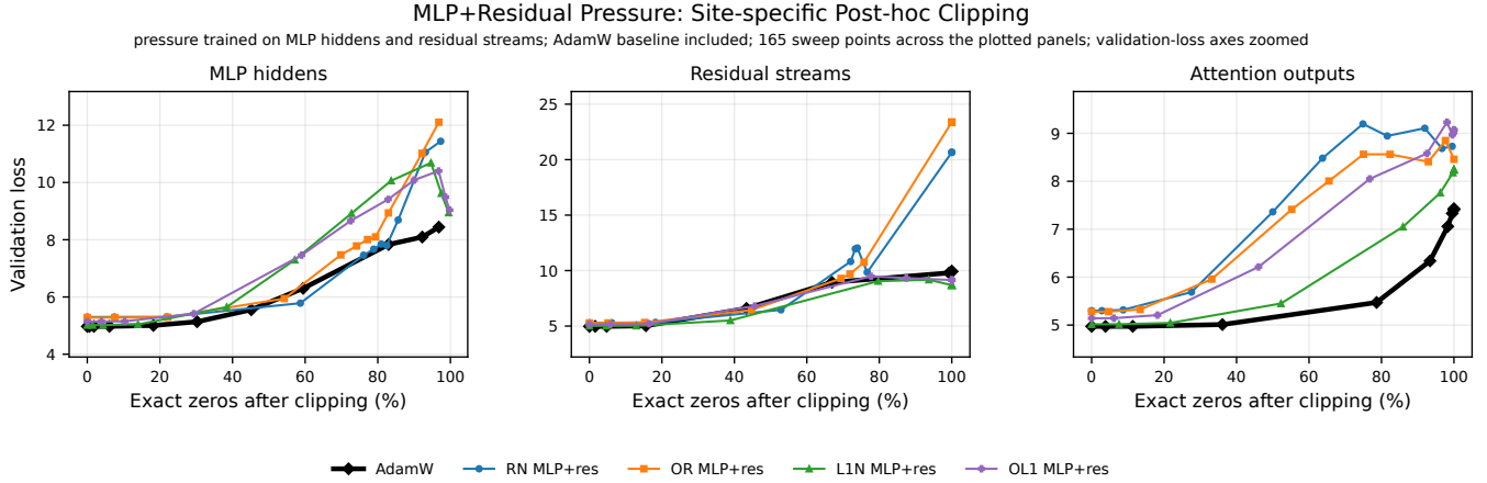
Figure 6: MLP+residual pressure post-hoc clipping frontiers in one comparable view, including the AdamW baseline. The site-wise view makes the tradeoff clearer: the best-loss L1N run no longer occupies the high MLP-sparsity regime, while residual and attention robustness differ by method.
