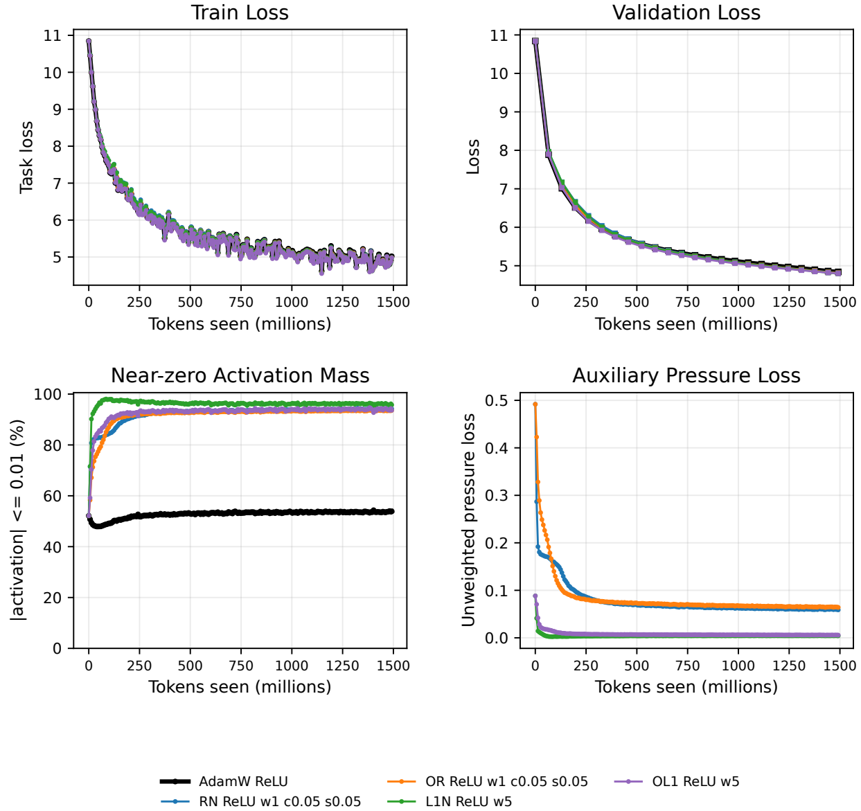
Figure 7: Completed ReLU learning curves for AdamW, RN, OR, L1N, and OL1.
