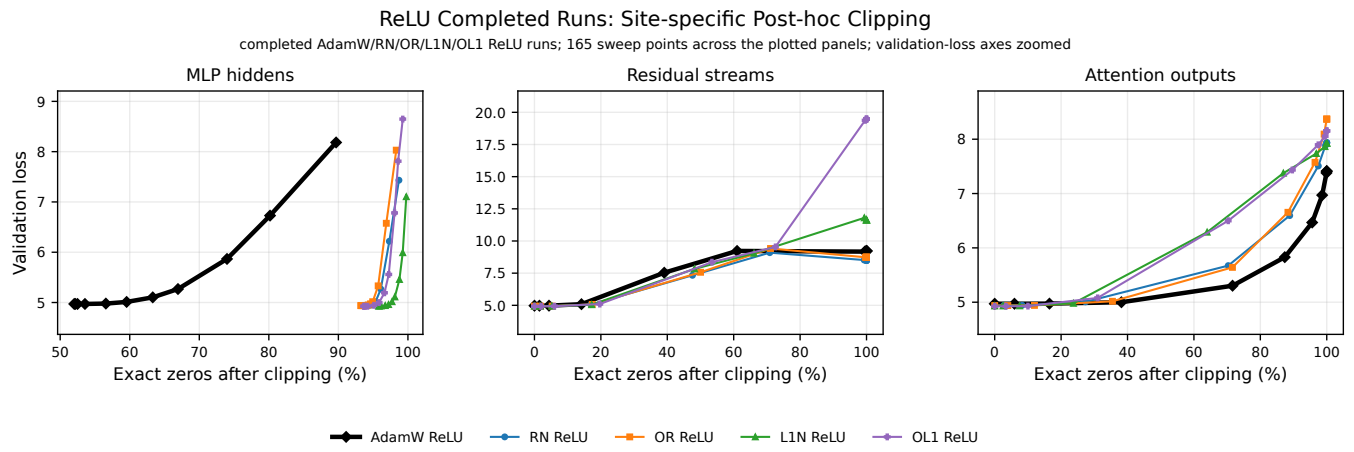
Figure 8: Completed ReLU post-hoc clipping frontiers in one comparable view. The MLP panel is the key activation-function result: RN, OR, L1N, and OL1 start near the high exact-zero regime with AdamW-level validation loss, unlike the GELU high-pressure tradeoff.
