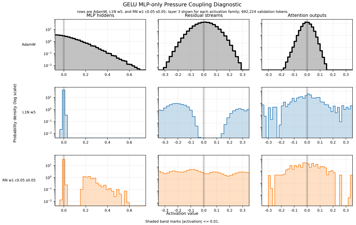
Figure 1: Compact activation-density coupling diagnostic for GELU MLP-only pressure, with log-scaled probability density. Rows compare AdamW, L1N w = 5 , and RN w = 1, c = 0.05, \sigma = 0.05 ; columns show MLP hidden, residual streams, and attention outputs at the same representative layer.
