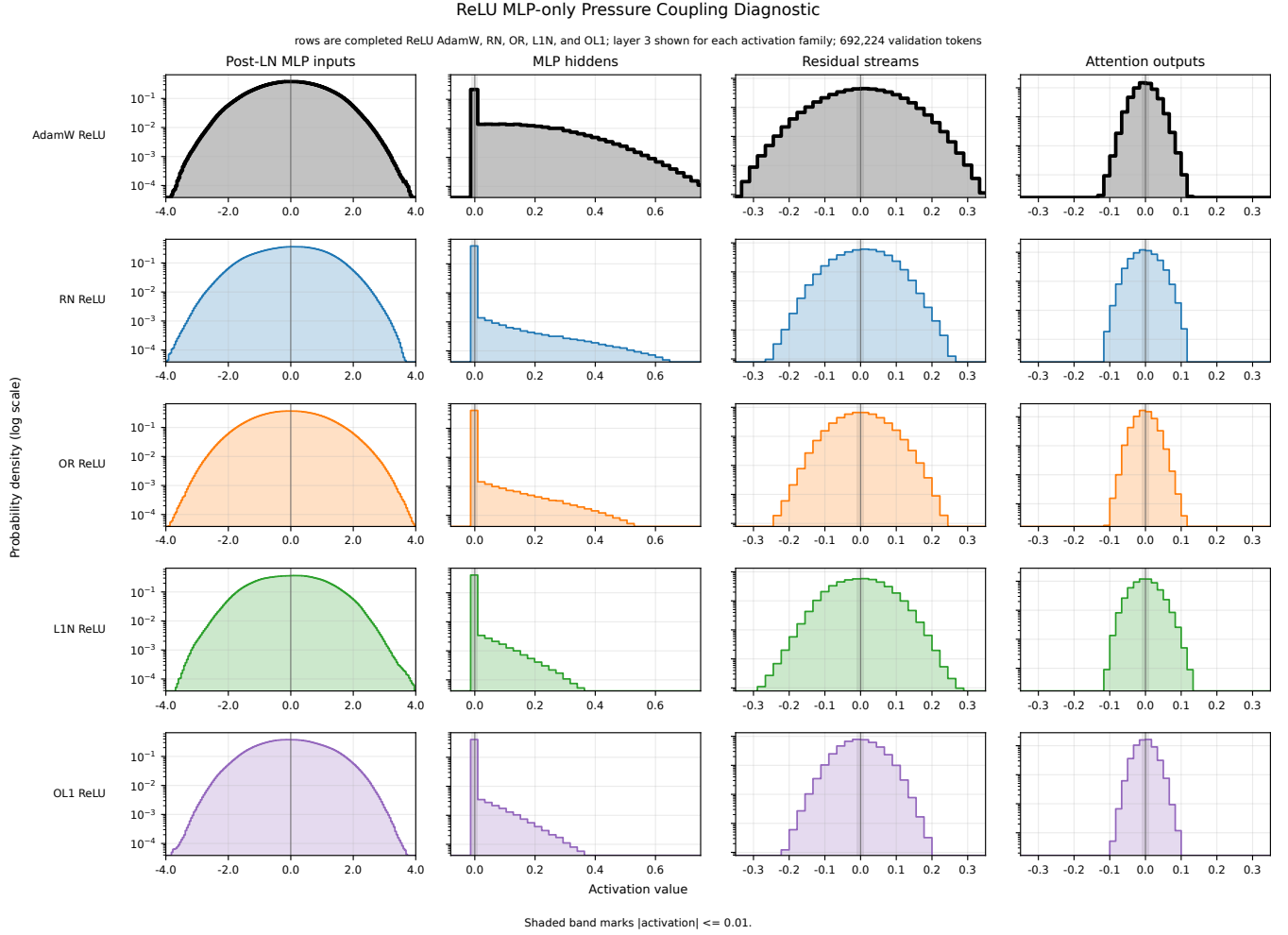
Figure 9: Completed ReLU coupling-density diagnostic. Rows compare AdamW, RN, OR, L1N, and OL1; columns add the post-LayerNorm MLP input density before the MLP-hidden, residual-stream, and attention-output densities.
