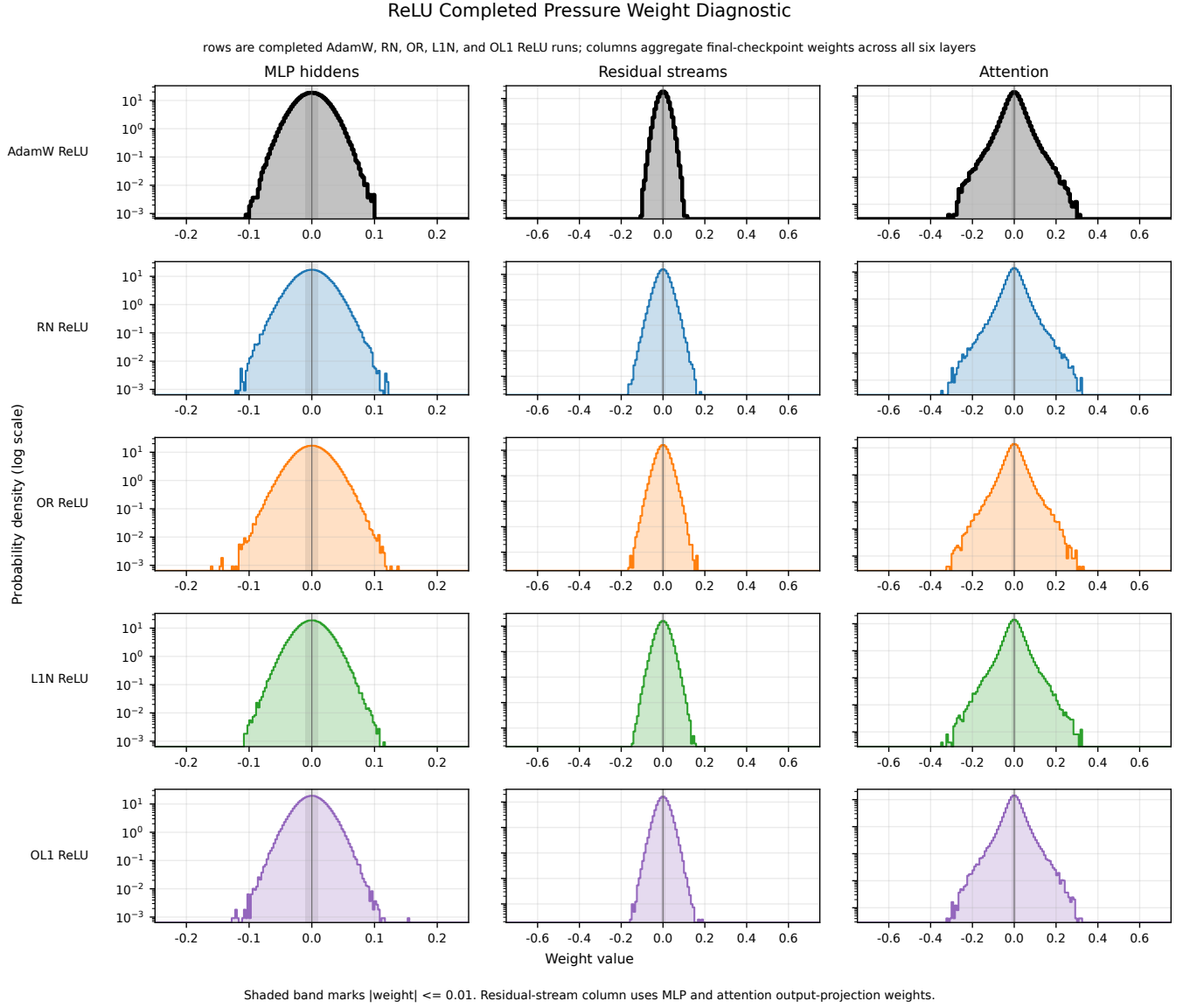
Figure 10: Completed ReLU pressure-weight diagnostic for AdamW, RN, OR, L1N, and OL1. Columns aggregate final-checkpoint weights across all six layers for MLP-hidden input weights, residual-stream output-projection weights, and attention QKV weights.
