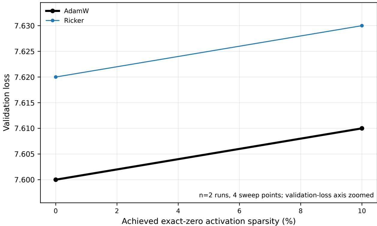
Post-hoc MLP Activation Clipping Frontiers
