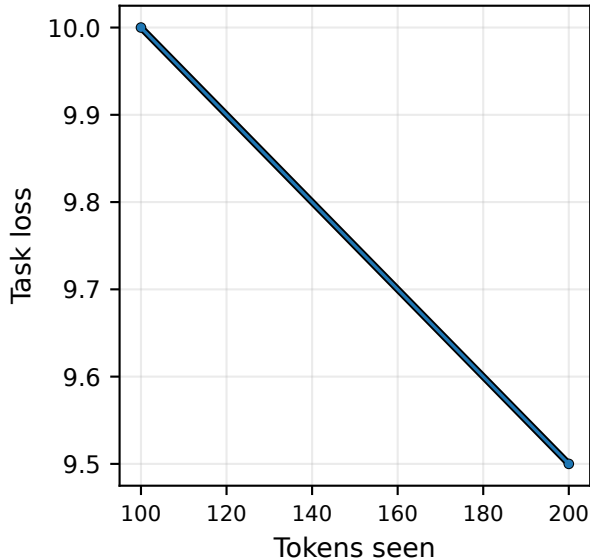
Train Loss
