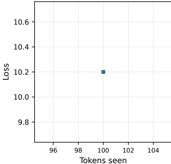
Validation Loss
