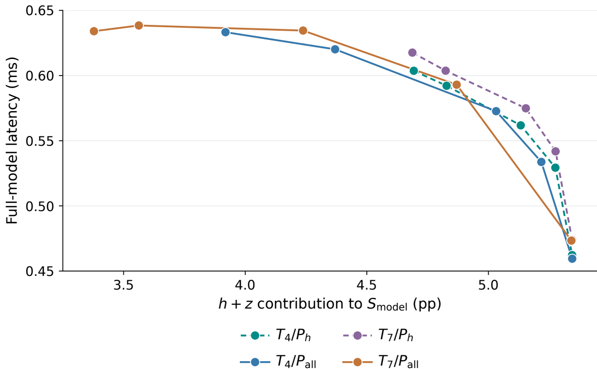
h, z sparsity contribution vs. latency on Pythia-14M
