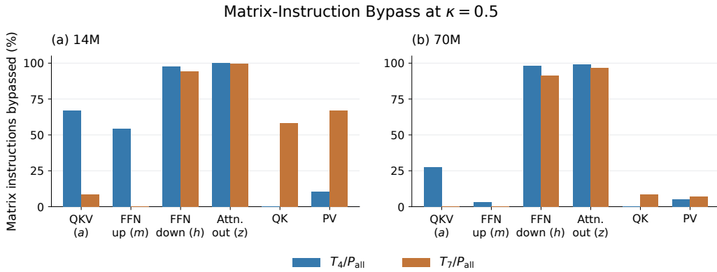
Figure 7: Instruction bypass does not guarantee lower latency. T_4/P_{\text{all}} and T_7/P_{\text{all}} at \kappa = 0.5 : (a) 14M; (b) 70M. Bars show bypassed divided by issued plus bypassed instructions per operation, pooled over all layers and 338 validation blocks. Bypass at h/z includes scalar replacements; attention counts include causal masking and padding. These percentages measure skipped instructions, not time saved.
