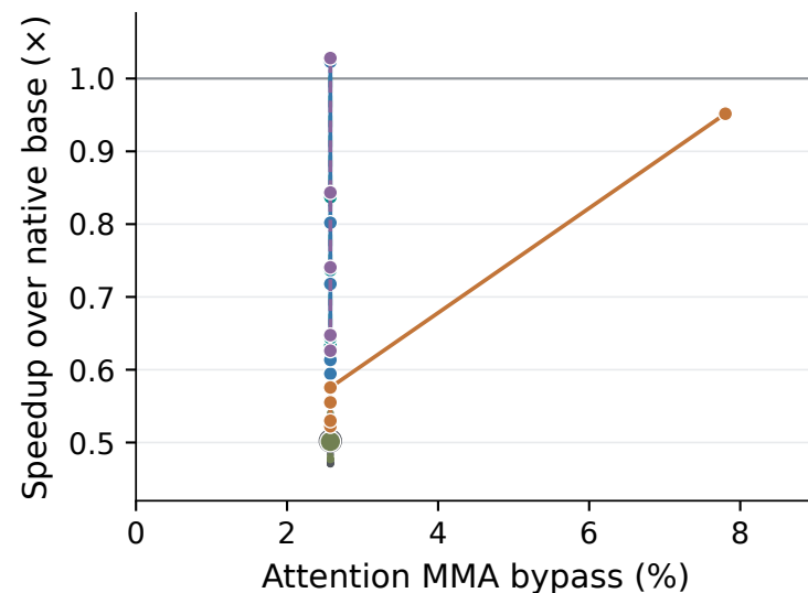
(f) 70M: Attention bypass and speedup
