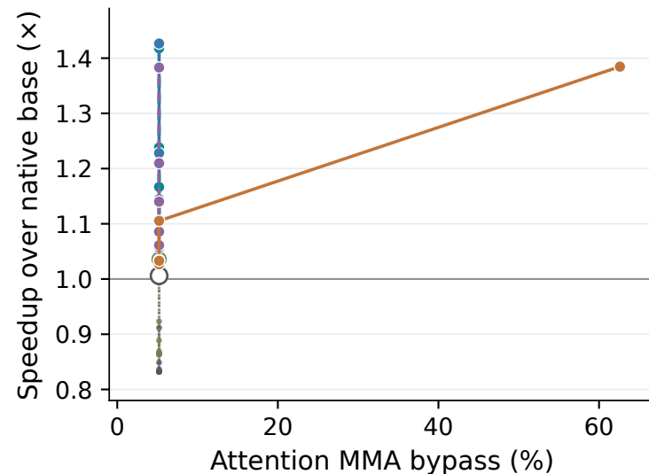
(c) 14M: Attention bypass and speedup
