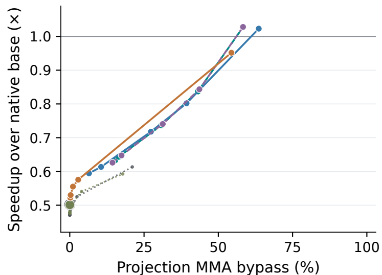
(e) 70M: Projection bypass and speedup
