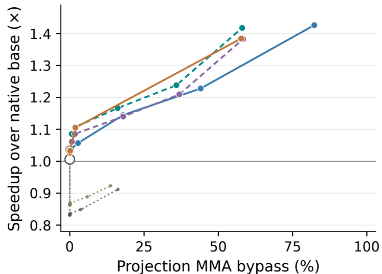
(b) 14M: Projection bypass and speedup
