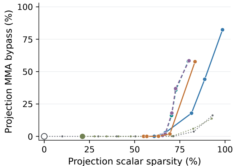
(a) 14M: Sparsity and bypass
