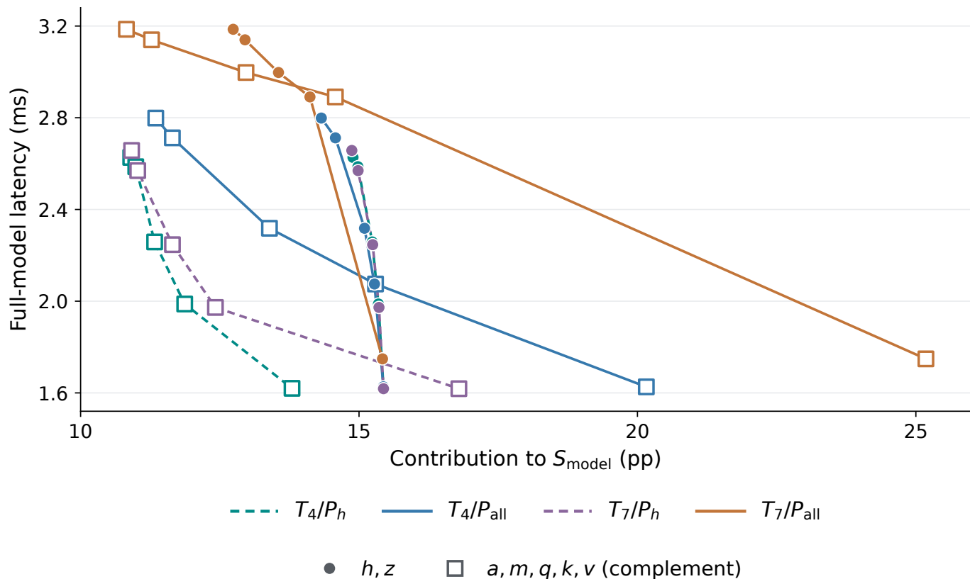
Sparsity contributions vs. latency on Pythia-70M
