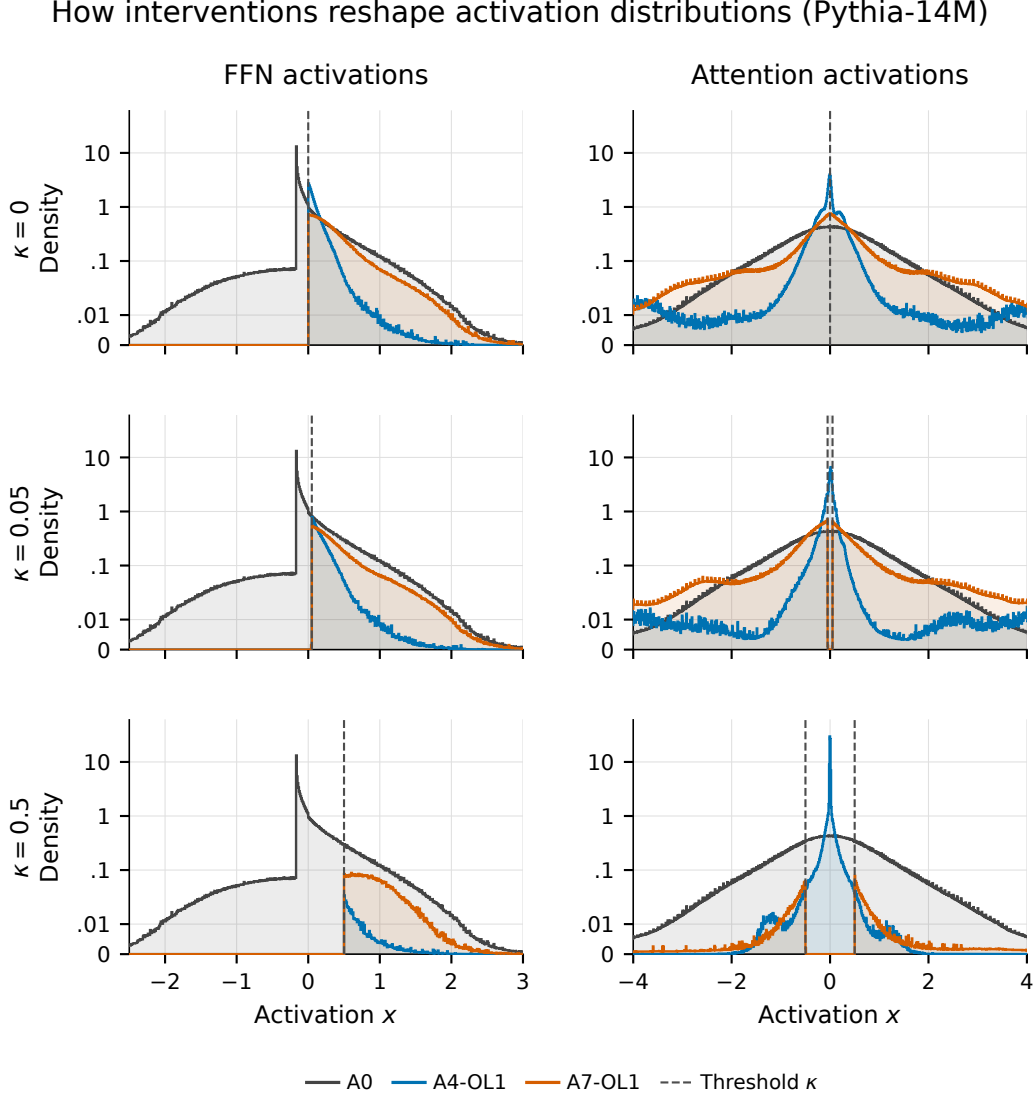
Figure 11: Interventions reshape FFN and attention distributions differently. Exact zeros are omitted from the curves and reported in Table 9. Columns pool FFN ( h, m ) and attention ( q, k, v ) activations; rows use trained thresholds \kappa = 0, 0.05, 0.5 . A0 is repeated across rows. Counts are pooled across all layers and validation blocks, weighting h : m by 80:20 and q : k : v equally. Density divides nonzero bin counts by all captured elements and bin width, without renormalizing the visible range. The vertical scale is symlog, linear below 0.01; filled areas on this scale do not represent probability mass. Dashed lines mark +\kappa for A4/A7 FFN thresholds and \pm\kappa for A7 attention thresholds. Q/K are measured after RoPE. A4 leaves q, k, v without direct thresholding or pressure; A7 targets them directly. The seven checkpoints use no additional post-hoc thresholding.
