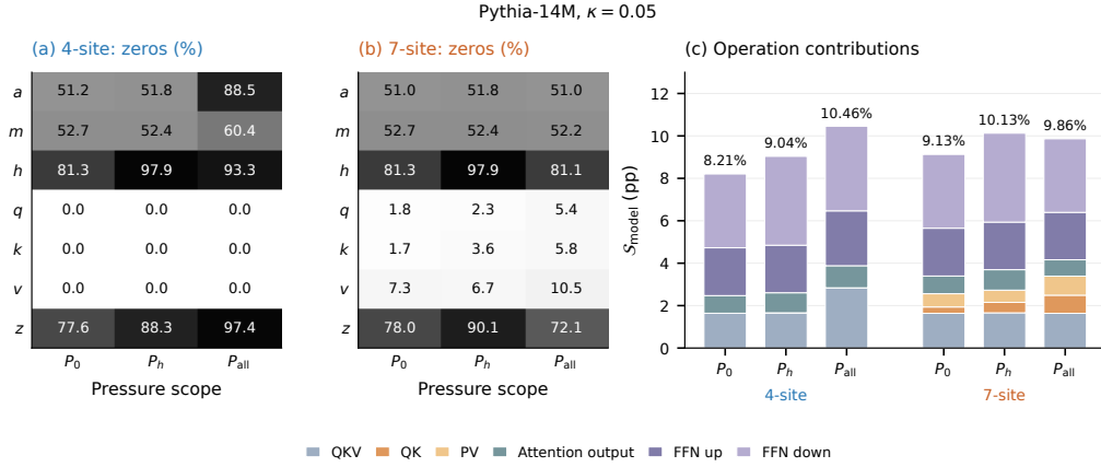
Figure 9: Pressure-scope effects at the moderate threshold \kappa = 0.05 . The six 14M recipes use the same count pooling and operation denominator as Figure 6. H-only pressure concentrates zeros at h while preserving a different pattern at m and Q/K/V from broad pressure. Rounded percentages do not establish all-zero or fully dense tensors.
