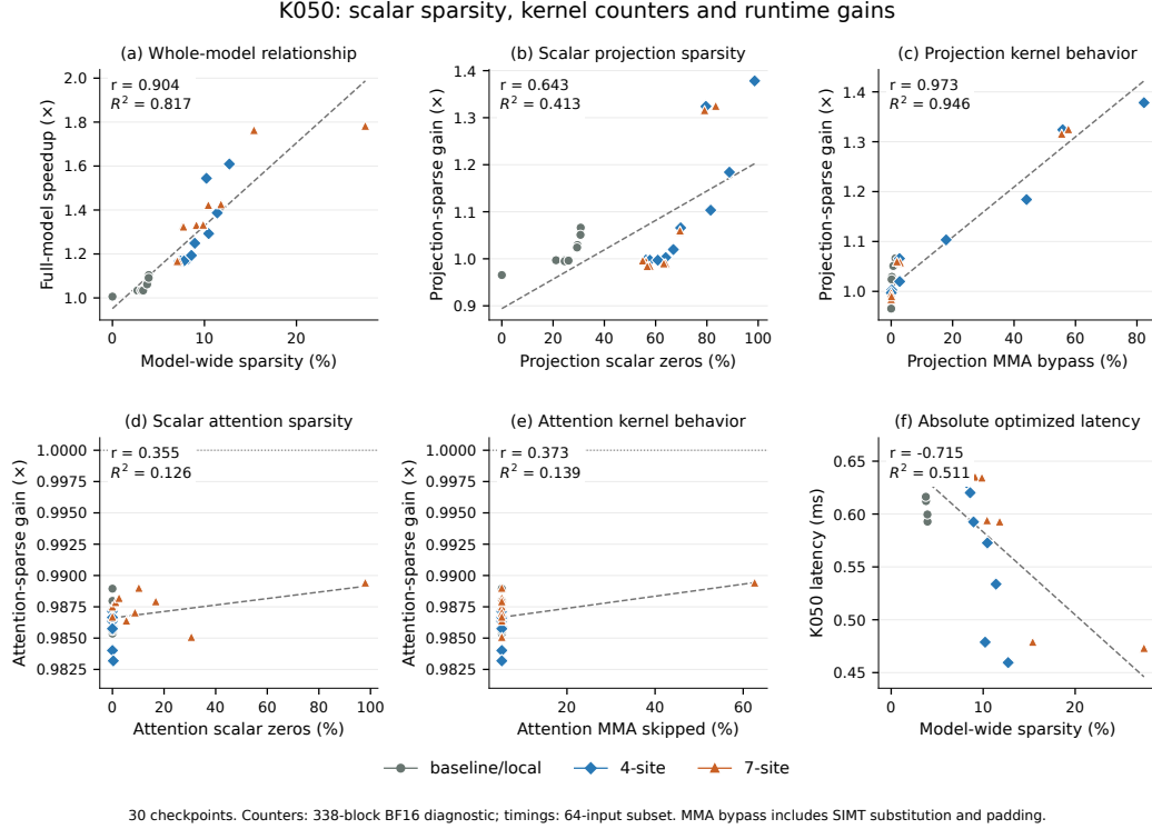
Figure 19: Scalar sparsity, skipped instructions, and matched runtime gains. The 30 checkpoints share colors and shapes by family. Projection and attention gains are t_0/t_P and t_P/t_K ; lines are descriptive OLS fits with intercepts. Projection bypass includes scalar substitution and padded MMA rows. Attention skip fractions include masked/padded work and take only two distinct values. The remaining pages of the accompanying diagnostic PDF show within-family fits, matched threshold comparisons, and absolute latency traces. Counters cover 338 validation blocks, while timings cover 64 matched inputs.
