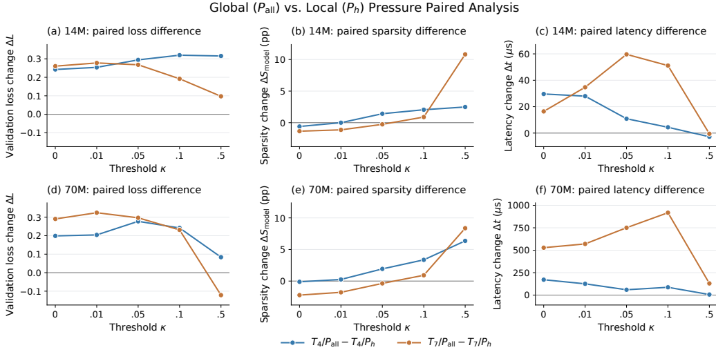
Figure 5: Paired effects of broadening pressure from P_h to P_{\text{all}} . Every point is all-site minus h-only pressure at matched model size, threshold scope and \kappa , with \lambda = b = 1 . Rows show 14M/70M; columns show loss change, sparsity change (pp), and full-model latency change ( \mu s ). Positive loss or latency differences favor P_h ; positive sparsity differences favor P_{\text{all}} . Latencies subtract checkpoint geometric means: RTX5090, BF16, batch one, 2,048 tokens, full logit head and 1,344 timings per checkpoint. The 14M T_7 pairs span GPU sessions; 70M uses the qualified K050 port. Small timing differences are descriptive. Lines connect separate single-seed runs with matched initialization, data order and training budget.
