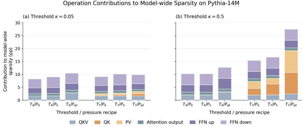
Figure 6: Where model-wide sparsity comes from. Operation contributions at 14M for \kappa = 0.05 (a) and \kappa = 0.5 (b), with P_0 , P_h and P_{all} under T_4/T_7 thresholding. Each segment is the operation’s zero-product count divided by the common full-model product count, in percentage points; stacks sum to 100S_{model} . Counts pool all layers and 338 complete validation blocks, including the dense output head in the denominator. These are logical opportunities, not measured time savings.
