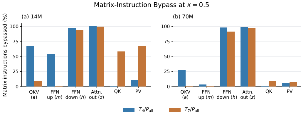
Figure 7: Skippable work is not the same as saved time. Matrix instructions bypassed for T_4/P_{all} and T_7/P_{all} at \kappa = 0.5 : (a) 14M and (b) 70M. Each bar pools bypassed instructions divided by issued plus bypassed instructions over all layers and complete validation. Labels identify each operation and its input site. Bypass at h/z includes replacement by a few scalar operations; attention counts include causal masking and padding. The bars do not measure latency or the fraction of total model work saved.
