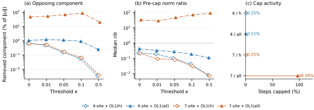
Figure 18: H-only and broad pressure operate in different norm-budget regimes at 14M. (a) Median removed opposing component, 100\rho_{\text{opp}} ; (b) median pre-cap ratio r/b at \lambda = b = 1 . Each point summarizes 712 optimizer steps at a fixed threshold, not seed uncertainty. Color denotes threshold scope; diamonds/dashed lines denote h-only pressure and triangles/dash-dot lines denote broad pressure. (c) Cap-active fractions pool 3,560 steps per recipe and use the implemented condition s < 1 . The geometry precedes group learning rates and decoupled weight decay, so it does not guarantee task-loss preservation. The h-only and broad-pressure comparison changes the objective composition and normalization.
