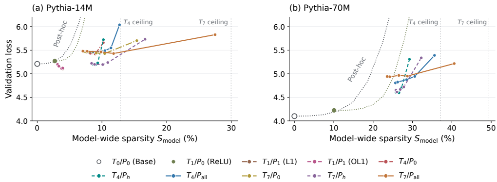
Quality-sparsity trade-offs on Pythia 14M and 70M
