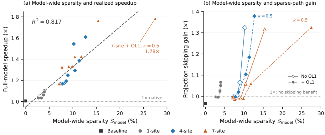
Figure 7: The runtime value of sparsity depends on where the zeros occur. (a) Native-relative full-model speedup of K050 across 30 Pythia-14M checkpoints versus \mathcal{S}_{\text{model}} . Marker shape identifies the intervention family; the dashed line is a descriptive OLS fit ( R^2 = 0.817 ). Seven-site + OL1 at \kappa = 0.5 reaches 1.78\times . (b) Gain from projection skipping versus \mathcal{S}_{\text{model}} : the geometric-mean latency with all skips disabled divided by that with projection skipping enabled, retaining the same fusion and disabled attention skipping. Values above 1\times indicate a net benefit. For four-/seven-site recipes, solid lines/open markers denote no OL1 and dashed lines/filled markers denote OL1. Lines connect separately trained thresholds in increasing order; muted gray paths connect the one-site L1/OL1 pressure-weight sweeps from ReLU. High thresholds produce substantial projection gains, further increased by OL1 for the four-site recipe. Seven-site OL1’s much larger \mathcal{S}_{\text{model}} does not yield a proportional projection gain: much of its additional sparsity occurs in QK/PV . Sparsity uses complete-validation FP16 counts; BF16 timing uses 64 matched inputs. These are descriptive associations across trained checkpoints, not causal effects of \mathcal{S}_{\text{model}} itself.
