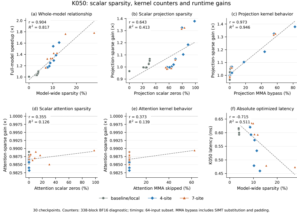
Figure 15: Scalar sparsity, skipped instructions, and matched runtime gains. The 30 checkpoints share colors and shapes by family. Projection and attention gains are t_0/t_P and t_P/t_K ; lines are descriptive OLS fits with intercepts. Projection bypass includes scalar substitution and padded MMA rows. Attention skip fractions include masked/padded work and take only two distinct values. The remaining pages of the accompanying diagnostic PDF show within-family fits, matched threshold comparisons, and absolute latency traces. Counters cover 338 validation blocks, while timings cover 64 matched inputs.
