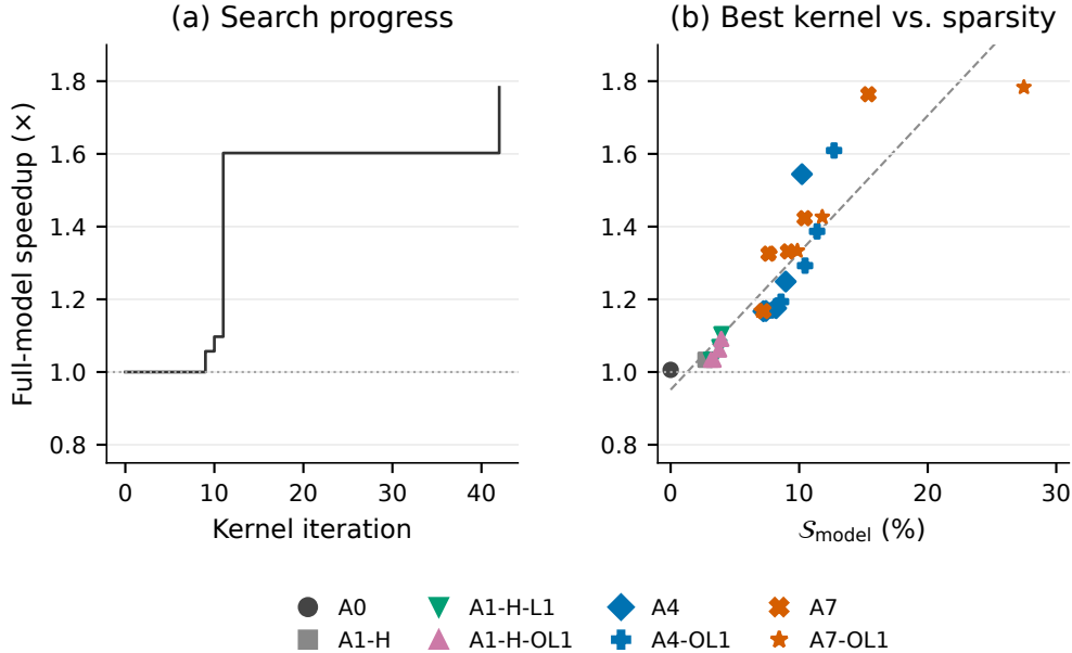
Figure 14: Kernel-search history and the final checkpoint sweep. (a) Best qualified incumbent across 42 eligible retrospective proposals on the fixed seven-site + OL1, \kappa = 0.5 checkpoint. (b) Final K050 speedup across the 30-checkpoint cohort; this historical view distinguishes individual recipes. Both use the same native PyTorch/SDPA CUDA-graph reference and BF16, batch-one, 2,048-token protocol on one RTX5090. Search replay and final evaluation are separate timing measurements. The history describes one human-guided development trajectory, not a comparison of coding agents.
