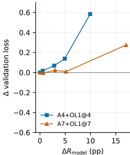
70M
