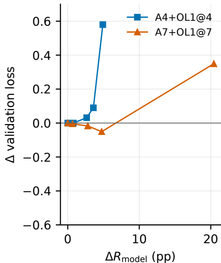
14M
