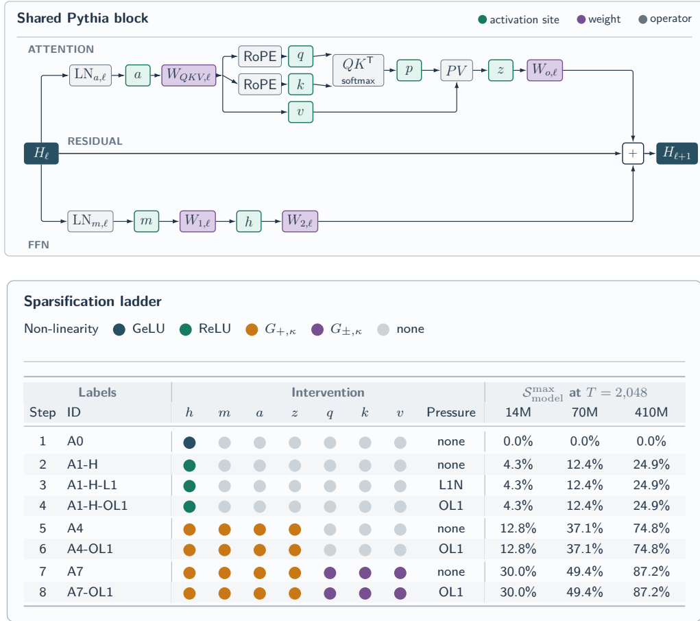
Figure 1: Shared Pythia block and sparsification intervention ladder. The map separates gate placement, gate family, and pressure; L1N denotes naive L1. The final columns show analytic selected-site reach 100 \mathcal{S}_{\text{model}}^{\max} % at T = 2,048 , not observed sparsity or speedup. Pressure targets all gated sites in each pressure-bearing row. Rows define candidate recipes; their experimental coverage is reported with the results.
