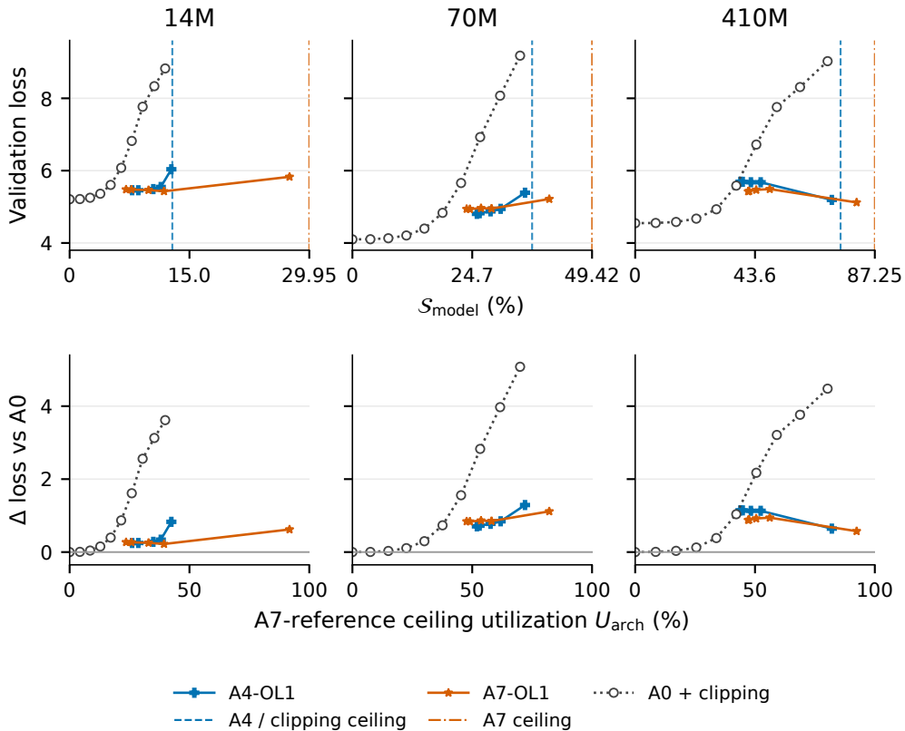
Quality vs. model-wide sparsity frontier across model sizes (Pythia-family)
