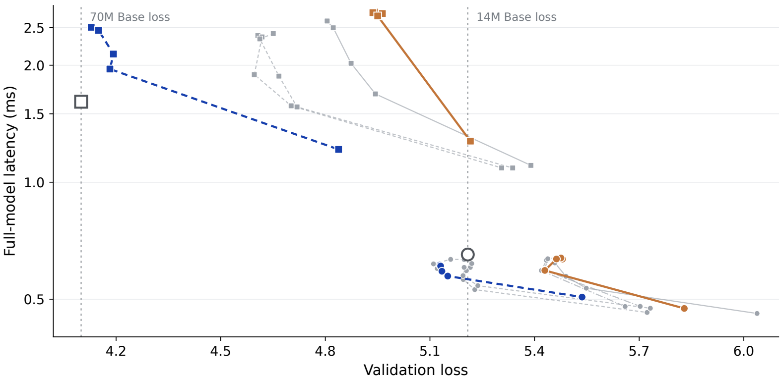
Pythia-14M and Pythia-70M
