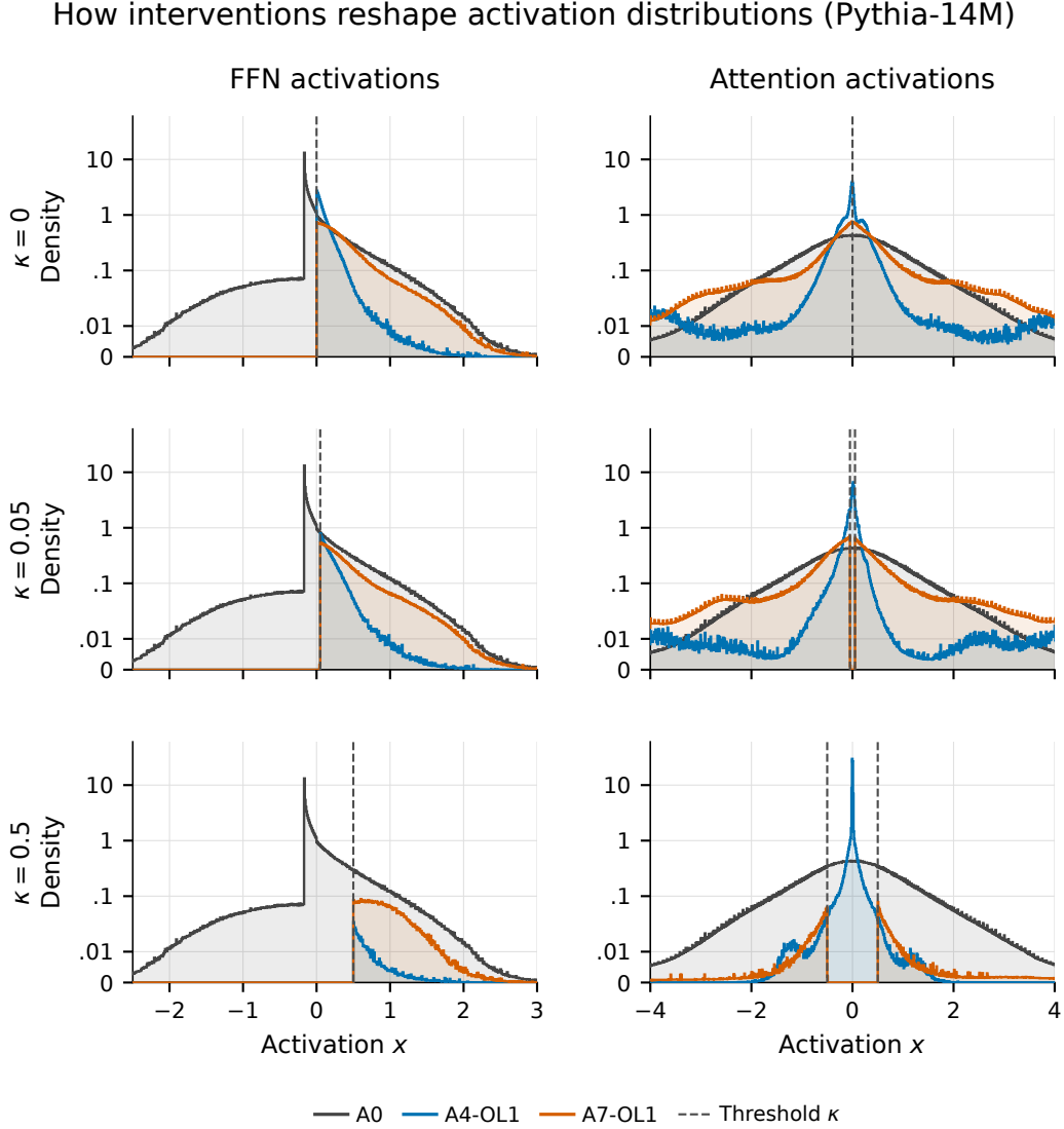
Figure 4: Interventions reshape FFN and attention distributions differently. Exact zeros are omitted from the curves and reported in Table 8. Columns pool FFN ( h, m ) and attention ( q, k, v ) activations; rows use trained thresholds \kappa = 0, 0.05, 0.5 . A0 is repeated across rows. Counts are pooled across all layers and validation blocks, weighting h : m by 80:20 and q : k : v equally. Density divides nonzero bin counts by all captured elements and bin width, without renormalizing the visible range. The vertical scale is symlog, linear below 0.01; filled areas on this scale do not represent probability mass. Dashed lines mark +\kappa for A4/A7 FFN thresholds and \pm\kappa for A7 attention thresholds. Q/K are measured after RoPE. A4 leaves q, k, v without direct thresholding or pressure; A7 targets them directly. The seven checkpoints use no additional post-hoc clipping.
