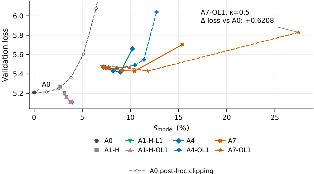
Quality-sparsity trade-offs for Pythia-14M
