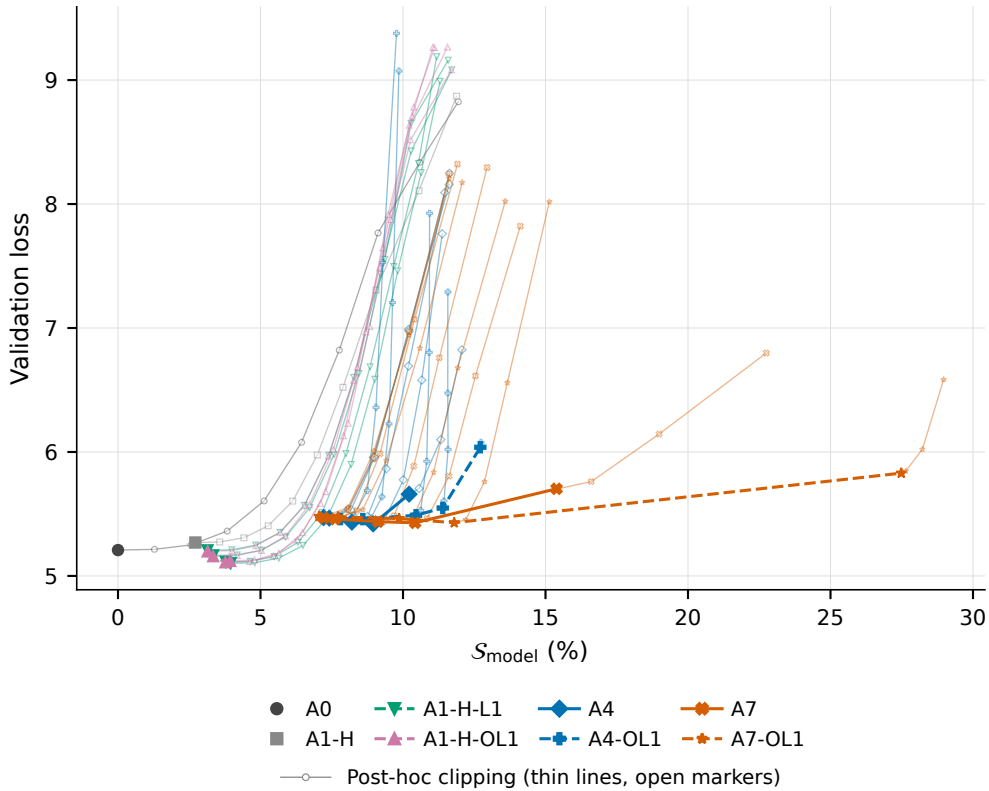
Figure 10: Complete 14M training and post-hoc clipping results: 30 trained endpoints and 300 clipping evaluations. Large filled markers denote trained endpoints; bold lines connect their settings, solid for unpressured recipes and dashed for L1/OL1. Each faint open-marker path follows one fixed checkpoint through p = 0, 0.1, \dots, 0.9 . Colors and symbols identify its source recipe. The full loss range is shown. Connections order evaluated settings and do not interpolate attainable models or fitted Pareto envelopes.
