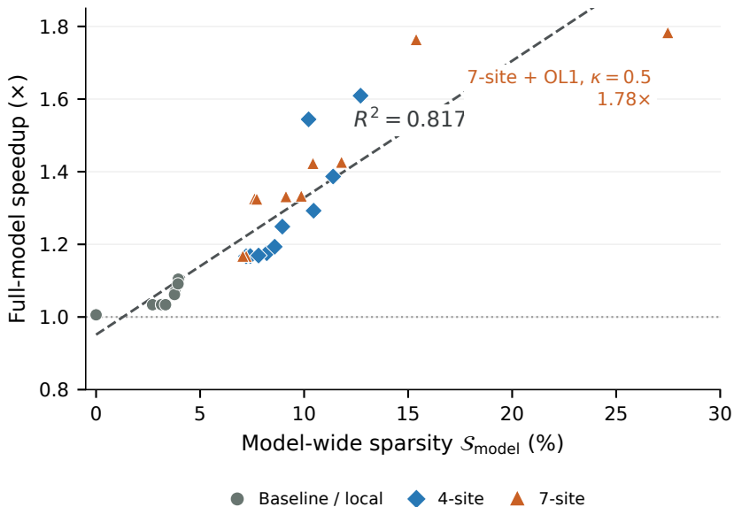
(a) Model-wide sparsity predicts realized speedup
