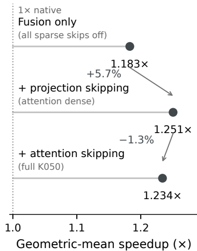
(b) Matched kernel ablations
