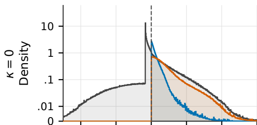
FFN activations
