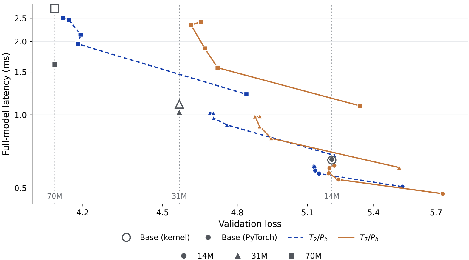
Quality-latency trade-offs across model scales
