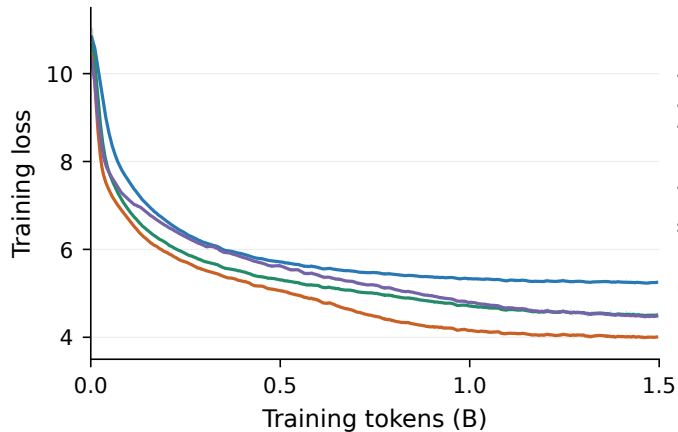
(a) T_0/P_0 training loss
