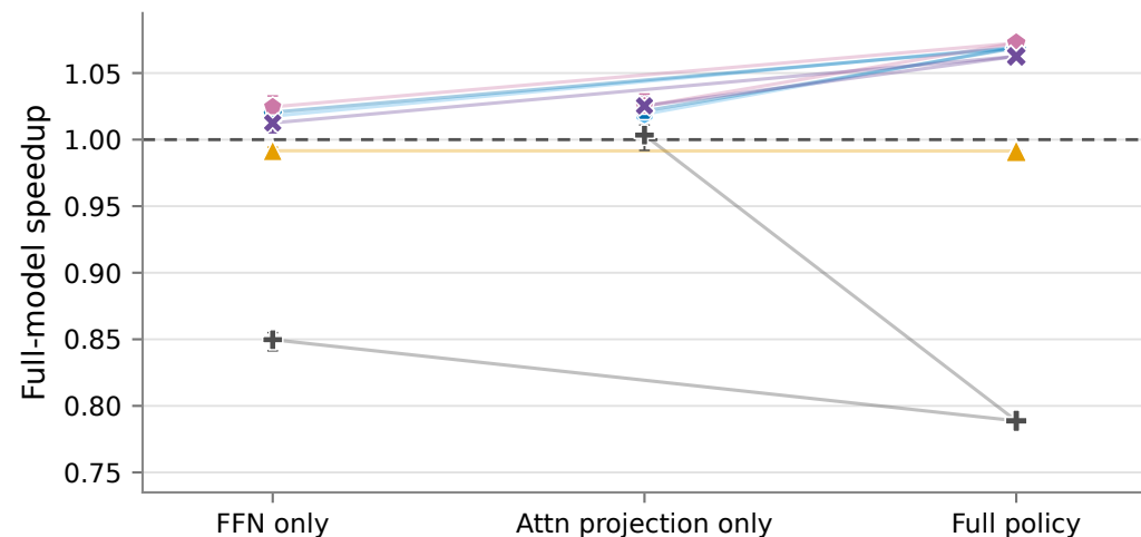
H100 NVL Hopper - Pythia-14M
