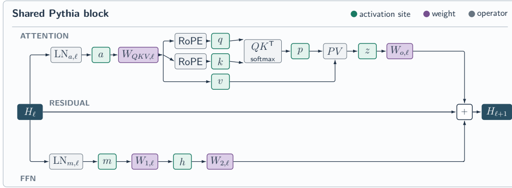
Figure 1: Intervention sites in a shared Pythia block. Attention and FFN branches use separate LayerNorms and join the residual path. Green nodes identify activation sites; purple nodes identify learned weights. Table 1 specifies thresholding and pressure assignments.
