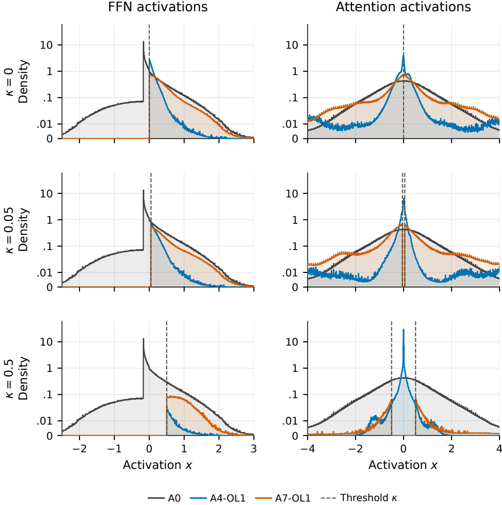
Figure 4: Interventions reshape FFN and attention distributions differently. Exact zeros are omitted from the curves and reported in Table 8. Columns pool FFN ( h, m ) and attention ( q, k, v ) activations; rows use trained thresholds \kappa = 0, 0.05, 0.5 . A0 is repeated across rows. Counts are pooled across all layers and validation blocks, weighting h : m by 80:20 and q : k : v equally. Density divides nonzero bin counts by all captured elements and bin width, without renormalizing the visible range. The vertical scale is symlog, linear below 0.01; filled areas on this scale do not represent probability mass. Dashed lines mark +\kappa for A4/A7 FFN thresholds and \pm\kappa for A7 attention thresholds. Q/K are measured after RoPE. A4 leaves q, k, v without direct thresholding or pressure; A7 targets them directly. The seven checkpoints use no additional post-hoc clipping.
