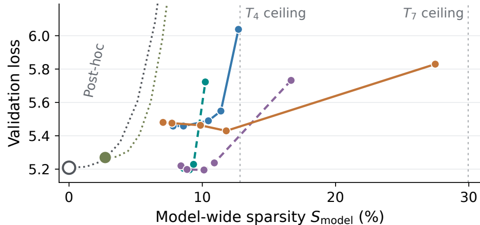
(a) 14M: quality-sparsity trade-off
