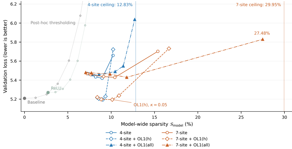
Figure 1: Threshold and pressure placement give distinct quality–sparsity trade-offs. Thirty multisite checkpoints span four-site (blue) and seven-site (orange) thresholding. Open circles/solid lines use no pressure; open diamonds/dashed lines use OL1 at h ; filled triangles/dash-dot lines use OL1 at all thresholded sites. Each curve joins five separately trained thresholds. Muted markers show A0 and ReLU; dotted paths apply post-hoc thresholding to those controls at a, m, h, z . Vertical guides show the selected-site ceilings. All 40 trained endpoints and the full historical post-hoc sweeps appear in the appendix.
