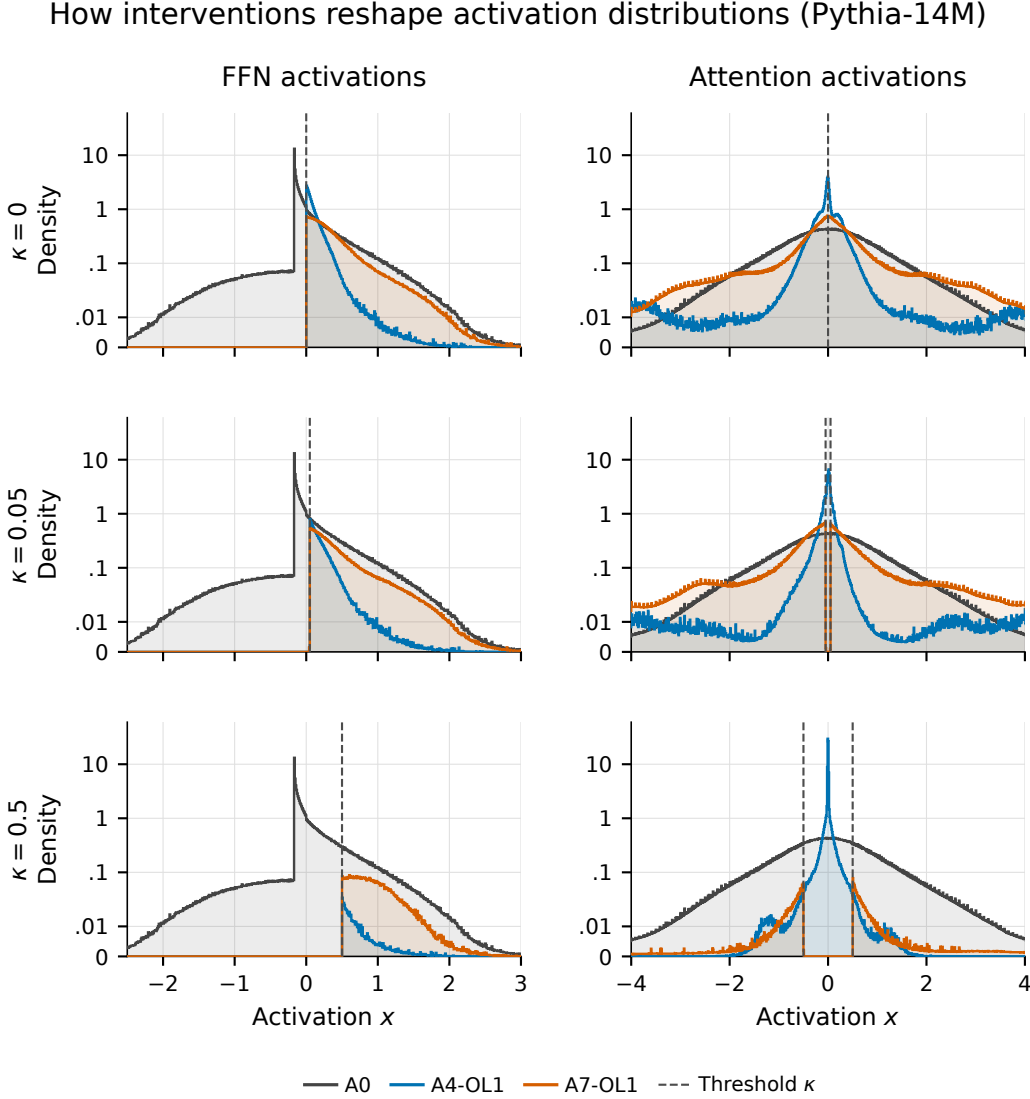
Figure 9: Interventions reshape FFN and attention distributions differently. Exact zeros are omitted from the curves and reported in Table 9. Columns pool FFN ( h, m ) and attention ( q, k, v ) activations; rows use trained thresholds \kappa = 0, 0.05, 0.5 . A0 is repeated across rows. Counts are pooled across all layers and validation blocks, weighting h : m by 80:20 and q : k : v equally. Density divides nonzero bin counts by all captured elements and bin width, without renormalizing the visible range. The vertical scale is symlog, linear below 0.01; filled areas on this scale do not represent probability mass. Dashed lines mark +\kappa for A4/A7 FFN thresholds and \pm\kappa for A7 attention thresholds. Q/K are measured after RoPE. A4 leaves q, k, v without direct thresholding or pressure; A7 targets them directly. The seven checkpoints use no additional post-hoc clipping.
