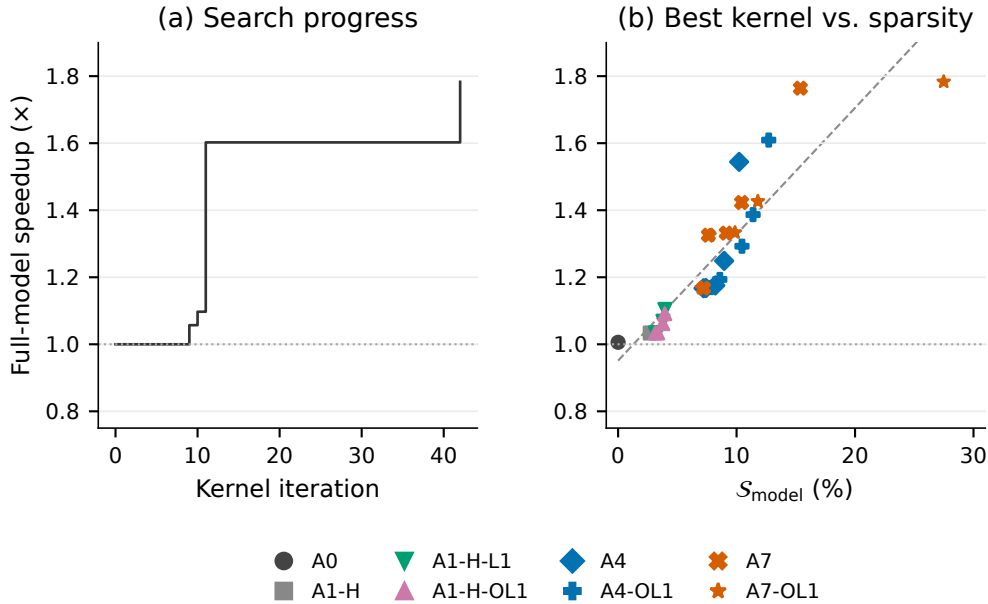
Figure 16: Kernel-search history and the final checkpoint sweep. (a) Best qualified incumbent across 42 eligible retrospective proposals on the fixed seven-site + OL1(all), \kappa = 0.5 checkpoint. (b) Final K050 speedup across the 30-checkpoint cohort; this historical view distinguishes individual recipes. Both use the same native PyTorch/SDPA CUDA-graph reference and BF16, batch-one, 2,048-token protocol on one RTX5090. Search replay and final evaluation are separate timing measurements. The history describes one human-guided development trajectory, not a comparison of coding agents.
