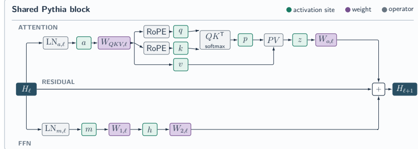
Figure 2: Intervention sites in a shared Pythia block. The attention and FFN branches use separate LayerNorms and join the residual path. Green nodes denote activation sites, and purple nodes denote learned weights. Table 1 specifies the thresholding and pressure assignments.
