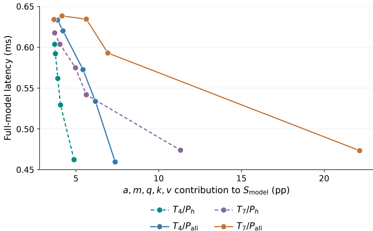
Sparsity outside h, z vs. latency on Pythia-14M
