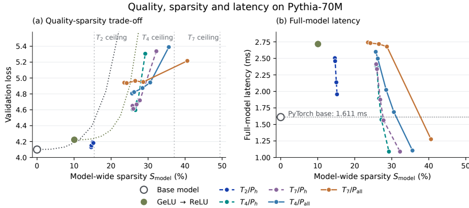
Figure 3: Quality, sparsity and execution on Pythia-70M. (a) Validation loss and (b) full-model latency versus \mathcal{S}_{\text{model}} for 26 matched checkpoints: Base, GeLU \rightarrow ReLU, T_2/P_h at \kappa = 0, .01, .05, .1 , and T_4/T_7 with P_h or P_{\text{all}} at \kappa = 0, .01, .05, .1, .5 . Colors and line styles match Figure 1. Dotted curves in (a) apply post-hoc clipping to the fixed Base/ReLU controls; high-loss tails extend beyond the view. Vertical guides mark sparsity ceilings. In (b), the Base marker and horizontal reference use native PyTorch/SDPA (1.611 ms); all other markers use the optimized 70M kernel. All 26 checkpoints share one RTX 5090 session, three fresh processes per checkpoint, batch one, 2,048 tokens and full output logits. Appendix E compares the native, original-port and optimized implementations. The additional T_2/P_h , \kappa = 0.5 endpoint is retained separately in Table 7.
