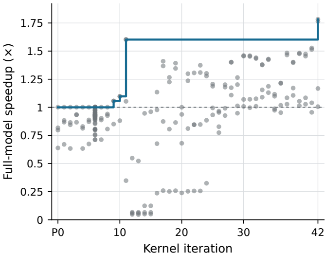
(a) Kernel auto-research progress
