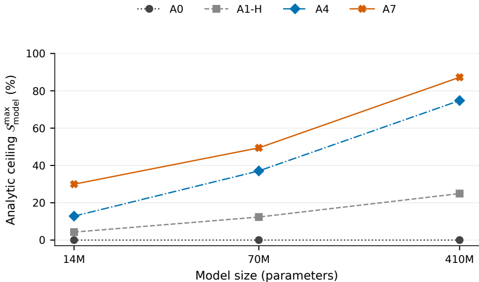
Theoretical sparsity ceiling by model size
