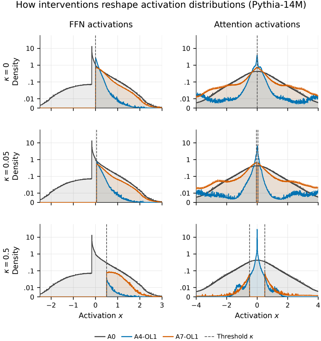
Figure 11: Interventions reshape FFN and attention distributions differently. Exact zeros are omitted from the curves and reported in Table 10. Columns pool FFN ( h, m ) and attention ( q, k, v ) activations; rows use trained thresholds \kappa = 0, 0.05, 0.5 . A0 is repeated across rows. Counts are pooled across all layers and validation blocks, weighting h : m by 80:20 and q : k : v equally. Density divides nonzero bin counts by all captured elements and bin width, without renormalizing the visible range. The vertical scale is symlog, linear below 0.01; filled areas on this scale do not represent probability mass. Dashed lines mark +\kappa for A4/A7 FFN thresholds and \pm\kappa for A7 attention thresholds. Q/K are measured after RoPE. A4 leaves q, k, v without direct thresholding or pressure; A7 targets them directly. The seven checkpoints use no additional post-hoc thresholding.
