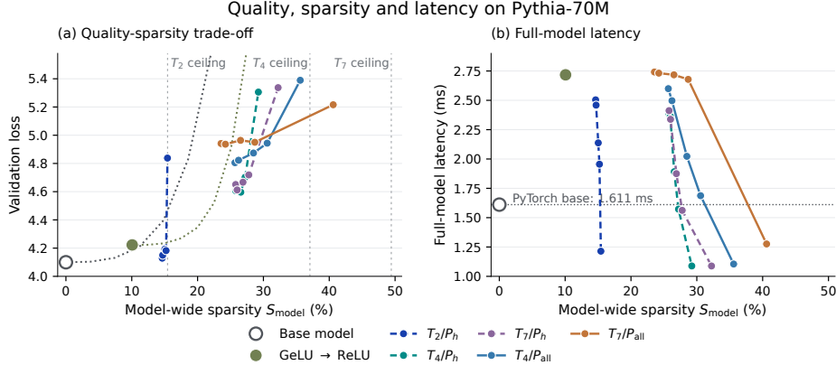
Figure 5: Quality, sparsity and execution on Pythia-70M. (a) Validation loss and (b) full-model latency versus S_{model} for 27 checkpoints: Base, GeLU \rightarrow ReLU, T_2/P_h , and T_4/T_7 with P_h or P_{all} , each thresholded recipe at \kappa = 0, .01, .05, .1, .5 . Colors and line styles match Figure 1. Dotted curves in (a) apply post-hoc clipping to the fixed Base/ReLU controls; high-loss tails extend beyond the view. Vertical guides mark sparsity ceilings. In (b), the Base marker and horizontal reference use native PyTorch/SDPA (1.611 ms); all other markers use the optimized 70M kernel. Measurements use RTX 5090 GPUs, three fresh processes per checkpoint, batch one, 2,048 tokens and full output logits. Appendix E compares the native, original-port and optimized implementations and reports the timing references.
