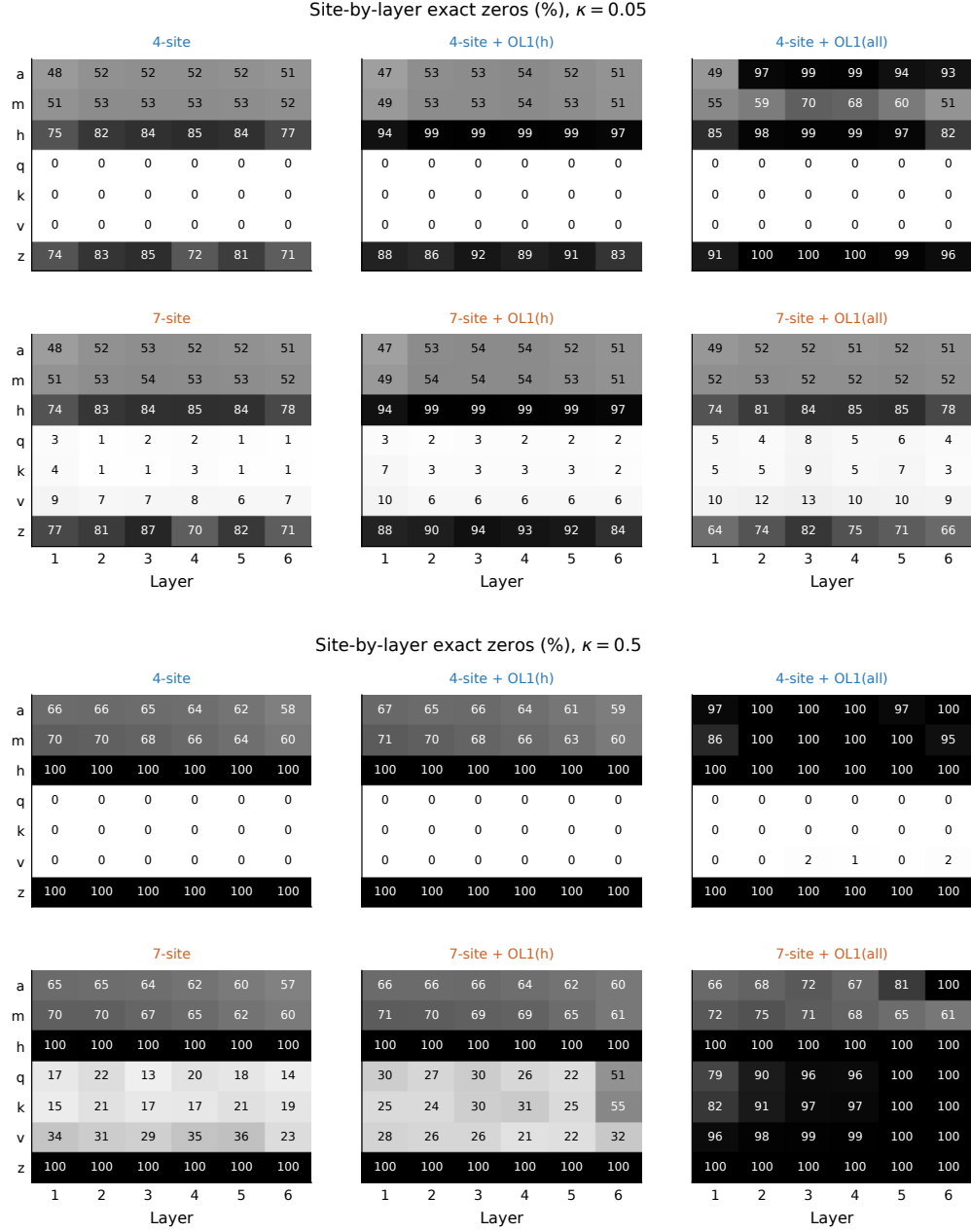
Figure 11: Site-by-layer zero fractions under matched pressure scopes. The six recipes at \kappa = 0.05 (top) and 0.5 (bottom). Each cell pools integer counts over all 338 validation blocks at one site and layer. Q/K are post-RoPE; values are rounded to whole percentages, so a displayed 100 does not imply an all-zero tensor. The complete five-threshold counters and source identities accompany the supplementary data.
