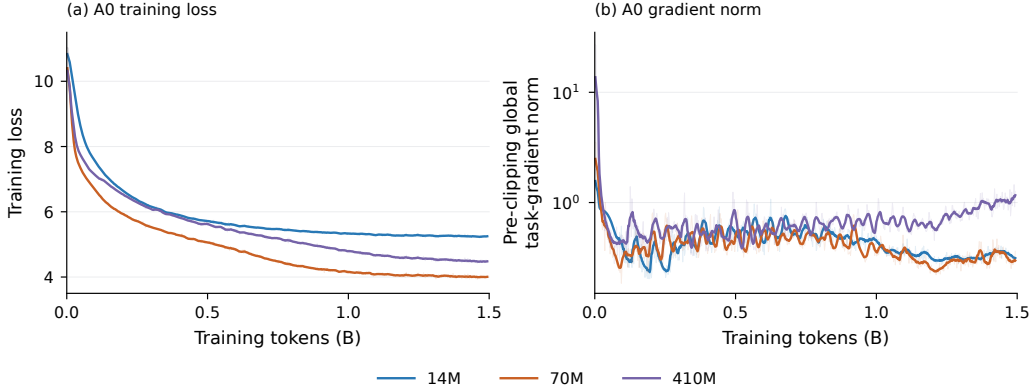
Figure 9: A0 optimization trajectories under the common training-token budget. (a) Training loss as a function of consumed input tokens for the 14M, 70M, and 410M A0 runs. (b) Pre-clipping global task-gradient norm over the same token budget; the logarithmic y-axis shows the large initial gradient transient and subsequent training regime. Faint traces show all 712 logged optimizer steps per size; opaque curves show a centered nine-step arithmetic moving mean, with partial windows at the edges. Norms are measured after loss unscaling and gradient accumulation, before clipping; smoothing is applied in the original units. All three sizes receive approximately 1.493B input tokens, but this corresponds to progressively fewer tokens per parameter as model size increases; the 410M run also uses a lower peak learning rate. Global norms are not normalized by parameter count. These trajectories characterize the realized optimization regimes and are not used as a convergence criterion.
