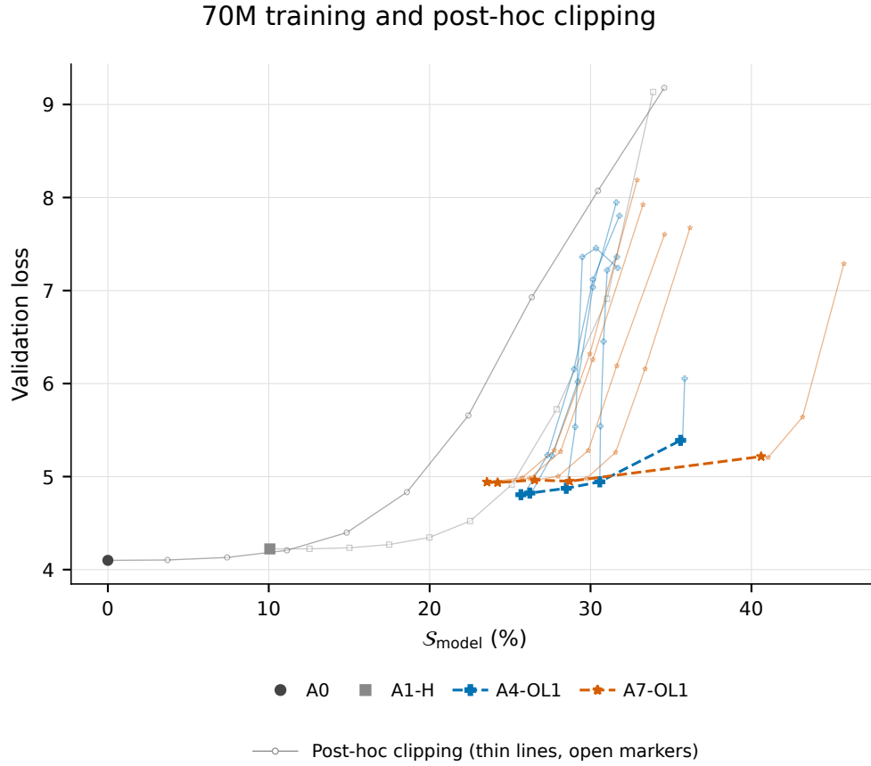
Figure 15: Complete 70M training and post-hoc thresholding results: 12 trained endpoints and 120 post-hoc thresholding evaluations. Large filled markers and bold lines identify the trained recipes; faint open-marker paths follow each checkpoint through ten increasing thresholding targets. All points, including overlaps and high-loss settings, are retained. The evaluation and line conventions match Figure 14.
