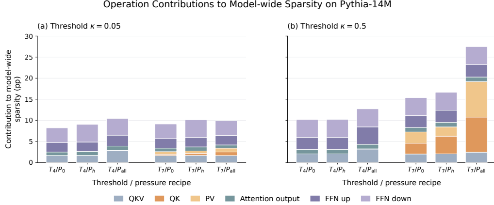
Figure 7: Where model-wide sparsity comes from. Operation contributions at 14M for \kappa = 0.05 (a) and \kappa = 0.5 (b), with P_0 , P_h and P_{\text{all}} under T_4/T_7 thresholding. Each segment is the operation’s zero-product count divided by the common full-model product count, in percentage points; stacks sum to 100\mathcal{S}_{\text{model}} . Counts pool all layers and 338 complete validation blocks, including the dense output head in the denominator. These are logical opportunities, not measured time savings.
