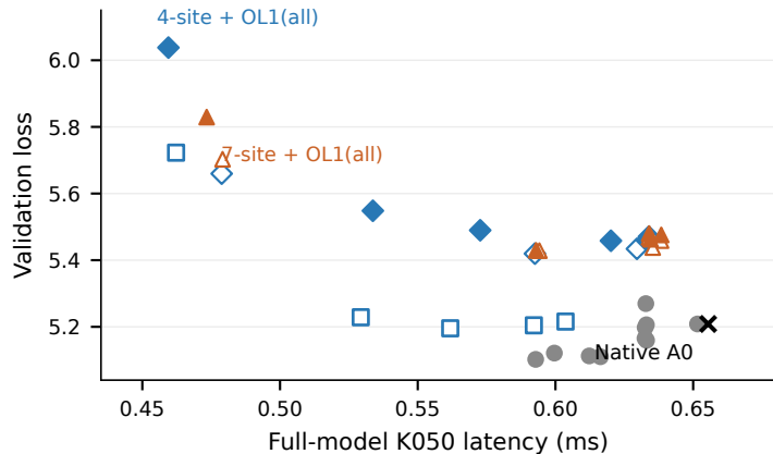
(a) Quality and absolute latency (35 models)
