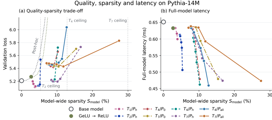
Figure 1: Quality, sparsity and execution on Pythia-14M. (a) Final validation loss and (b) full-model latency versus S_{\text{model}} for the same 41 checkpoints: the Base Model ( T_0/P_0 ), GeLU \rightarrow ReLU ( T_1/P_0 ), T_1/P_h , T_2/P_h with thresholds at h , z , and T_4/T_7 with no pressure ( P_0 , dash-dot), pressure at h ( P_h , dashed), or pressure at all thresholded sites ( P_{\text{all}} , solid). Curves connect separate trained settings: \lambda = .05, .1, .5, 1 for T_1/P_h ; \kappa = 0, .01, .05, .1, .5 for T_2/P_h ; and \kappa = 0, .01, .05, .1, .5 for T_4/T_7 . Dotted curves in (a) show post-hoc clipping of the Base/ReLU controls at p = 0, .1, \dots, .9 ; high-loss tails extend beyond the view. Panel (b) shows trained checkpoints only. Vertical dotted lines mark analytic sparsity ceilings. Latencies use RTX5090, batch one and 2,048-token sequences.
