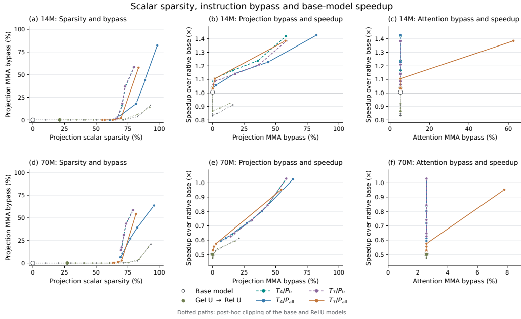
Figure 10: Scalar sparsity, instruction bypass and speedup over a fixed native base model. Rows show 14M and 70M, each with 22 trained settings and 20 post-hoc control settings. Left: projection scalar sparsity versus projection MMA bypass. Middle/right: projection/attention bypass versus full-model speedup. Every speedup within a row uses the same native T_0/P_0 reference; the horizontal line is 1\times . The Base model marker uses specialized inference, so it need not lie on that line. Lines connect measured thresholds, not fitted trends; dotted paths are post-hoc clipping. Counts are pooled, include the instruction-padding and scalar-substitution conventions above, and do not measure saved memory traffic.
