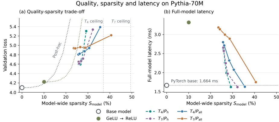
Figure 3: Quality, sparsity and execution on Pythia-70M. (a) Validation loss and (b) full-model latency versus S_{\text{model}} for 22 trained checkpoints: Base, GeLU \rightarrow ReLU, and T_4/T_7 with P_h or P_{\text{all}} at \kappa = 0, .01, .05, .1, .5 . Colors and line styles match Figure 1. Dotted curves in (a) apply post-hoc clipping to the fixed Base/ReLU controls; high-loss tails extend beyond the view. Vertical guides mark sparsity ceilings. In (b), the Base marker and horizontal reference use native PyTorch/SDPA (1.664 ms); all other markers use the original 70M port of the 14M kernel. All trained timings use the same RTX 5090 session, batch one, 2,048 tokens and full output logits. Later optimization results are reported separately in Appendix E.
