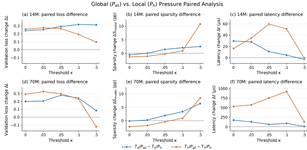
Figure 4: Paired effects of broadening pressure from P_h to P_{all} . Every point is P_{all} minus P_h at matched model size, threshold sites and \kappa , with \lambda = b = 1 . Rows show 14M/70M; columns show loss change, sparsity change (pp), and full-model latency change ( \mu s ). Positive loss or latency differences favor P_h ; positive sparsity differences favor P_{all} .
